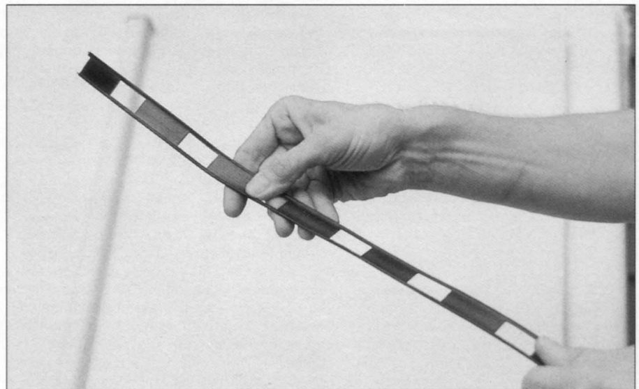
Fig 1 —This type of 450-ohm ladder line uses plastic insulating material to maintain a consistent separation between the two conductors. The air gaps between the insulation gives it its ladder-like appearance. Other types of open-wire line are available, but 450-ohm ladder line is the most common.
