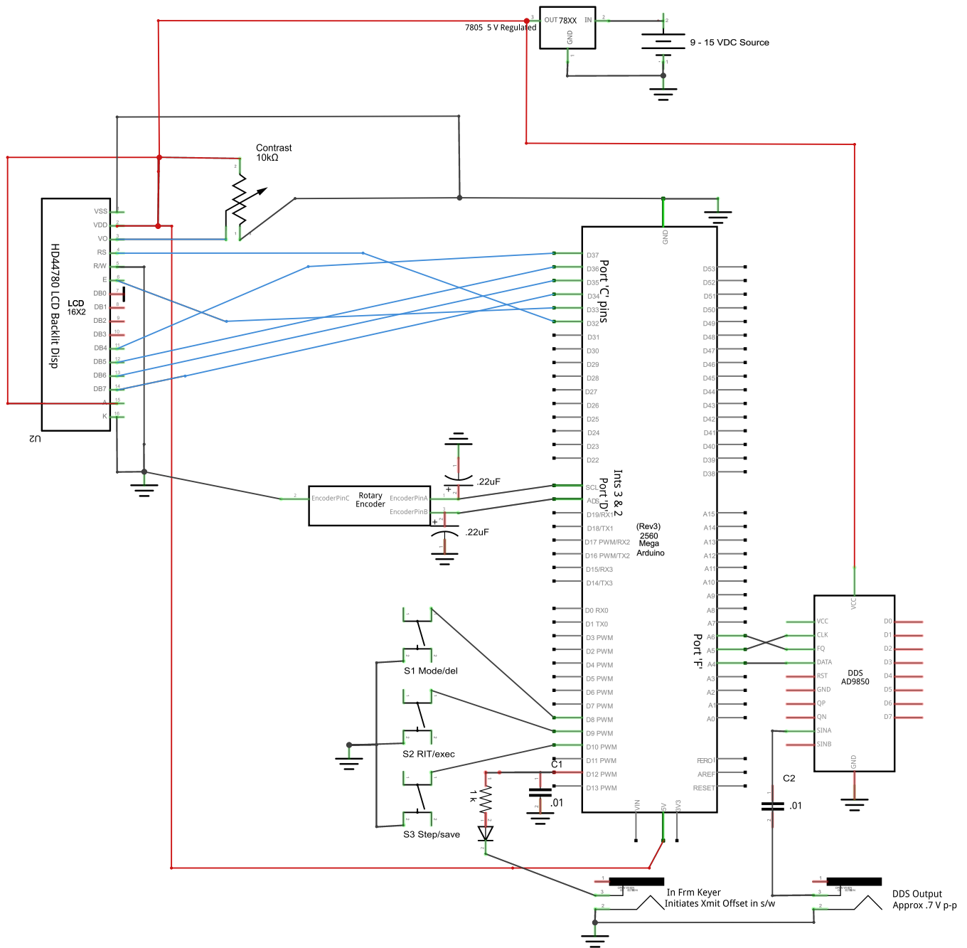
Arduino Mega 2560 Controlled AD9850 DDS VFO R.L.Snow 11/13/2015 Rev 1.0
