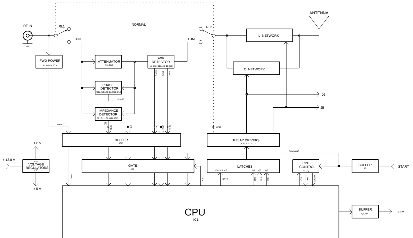
AH-3 BLOCK DIAGRAM
