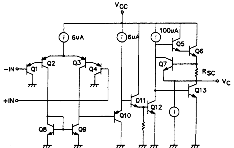
Equivalent Circuit
