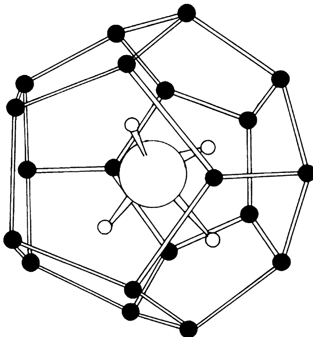
Fig. 6.3 Model of part of a methane-hydrate cell showing the oxygen atoms (•) of the water molecules with the \text{CH}_4 in the center
