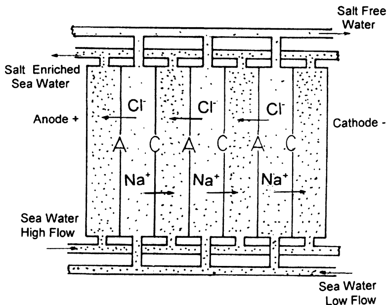
Fig. 15.7 Schematic representation of the desalination of water by electrodialysis. “A” refers to the anion-exchange membrane, and “C” refers to the cation-exchange membrane. The applied voltage attracts the ions from the low-flow water stream into the high-flow wastewater
