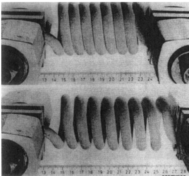
Fig. 17.2 Coiled high-strength micro-defect-free (MDF) cement spring in relaxed and extended positions
