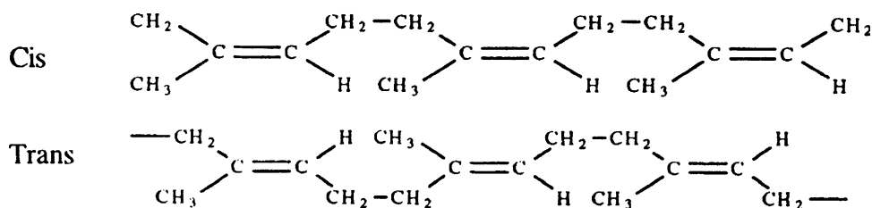
Fig. 11.9 Structures of natural rubber: cis , natural, herea and trans ; gutta, percha, balata
