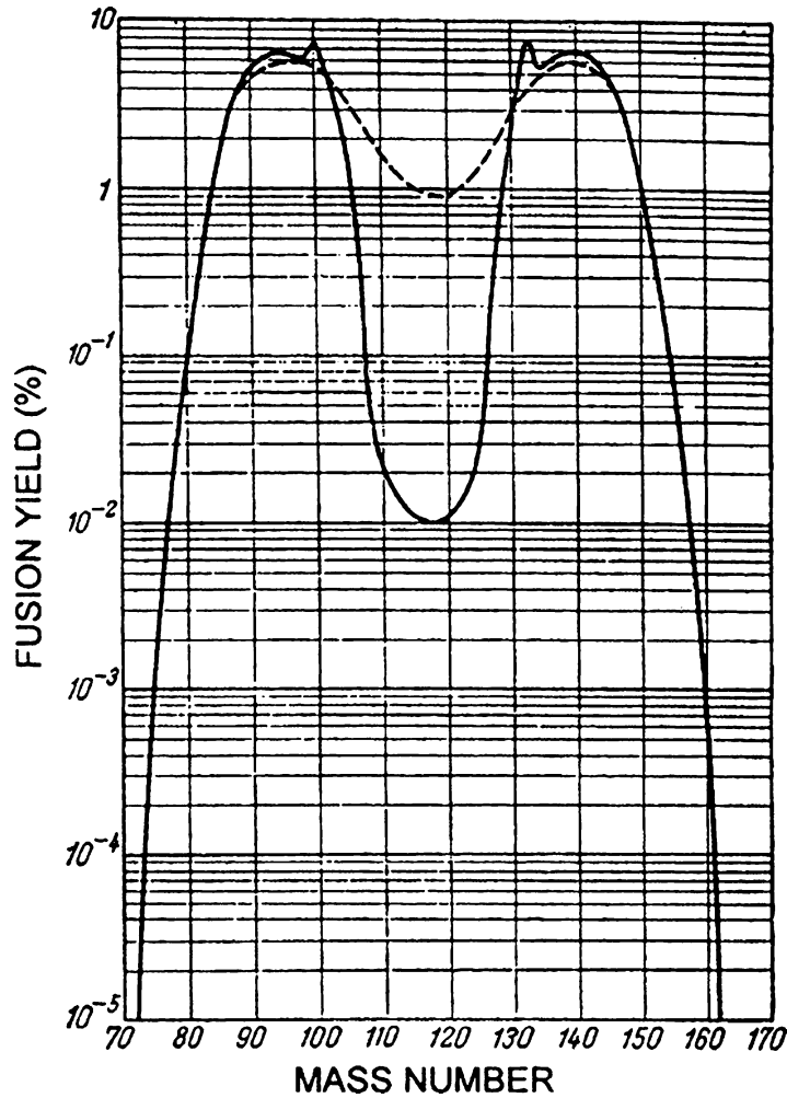
Fig. 7.4 The distribution of fission products from the reaction of ^{235}_{92}\text{U} with slow neutrons
