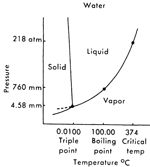
Fig. 15.2 The 2-D phase diagram of water showing the triple point, critical temperature, and critical pressure
