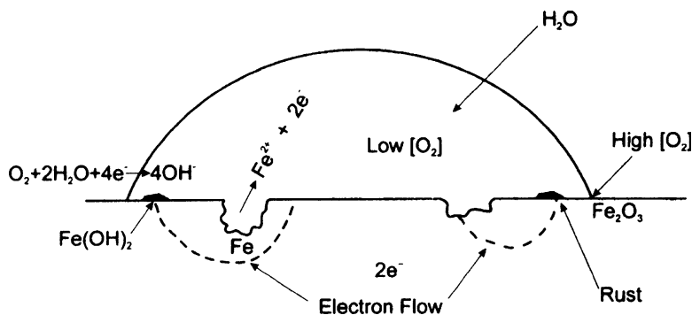
Fig. 10.2 A gradient in O 2 concentration in the water drop makes the center portion of the iron anodic where \text{Fe} \rightarrow \text{Fe}^{2+} + 2\text{e}^- , while the edge is cathodic and oxygen is reduced
