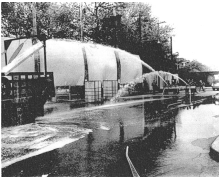
Fig. B.6 Effect of high molecular weight polyethylene oxide) in increasing water flow through fire hoses. Hoses had been adjusted to throw water the same distance and then 30 ppm of polyethylene oxide) were injected into the hose on the left
