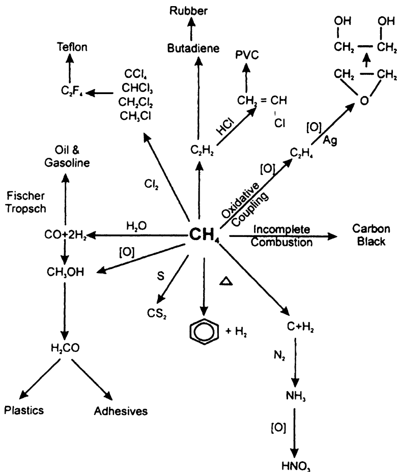
Fig. 6.4 Chemical reactions and uses of methane
