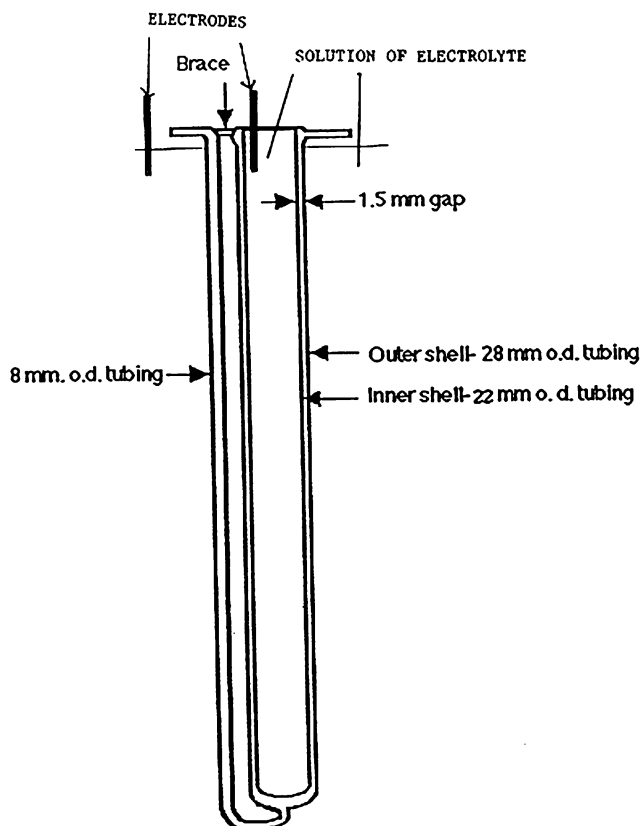
Fig. 15.5 Silent discharge reactor tube for ozone production. The tube is filled with electrolyte and placed in a container full of electrolyte solution which holds the high-voltage ac electrodes. The electrolyte is usually copper sulfate or sodium sulfate in water. The electrodes are usually copper
