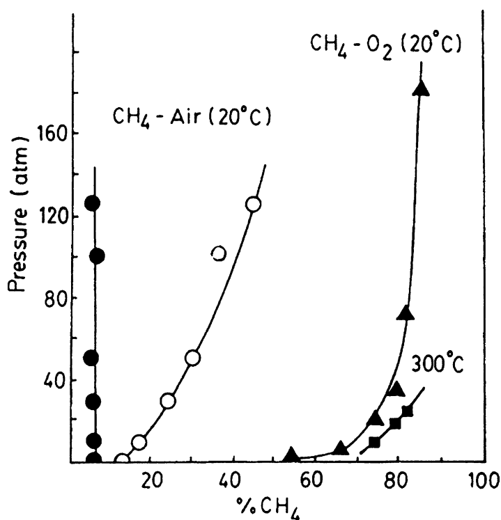
Fig. 6.7 Explosion limits for CH_4 in air (circles, ● and ○) and in O_2 , filled points, ● and ▲ at 20°C and for CH_4 in O_2 at 300°C (● and ■)
