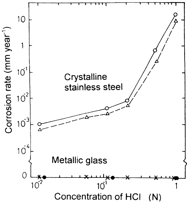
Fig. 10.3 A comparison of the corrosion rates of metallic glasses (x,●) and crystalline stainless steel (O, Δ) as a function of HCl concentration at 30°C. No weight changes of the metallic glasses of Fe-Cr 10 P 13 C 7 were detected by a microbalance after immersion for 200 hr
