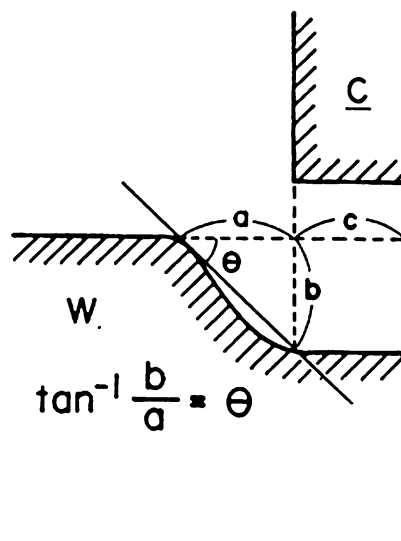
Fig. 9.6 Schematic diagram of machined surface (see Figs. 9.3, 9.4, and 9.5). W working electrode (15 mmφ), C counter electrode (5 mmφ), θ machined angle
