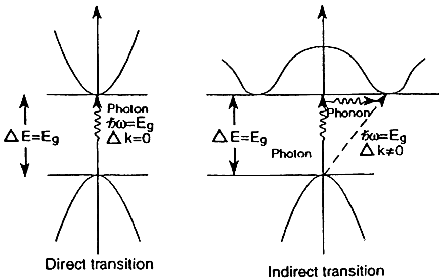
Fig. 18.4 Direct and indirect band gaps in semiconductors
