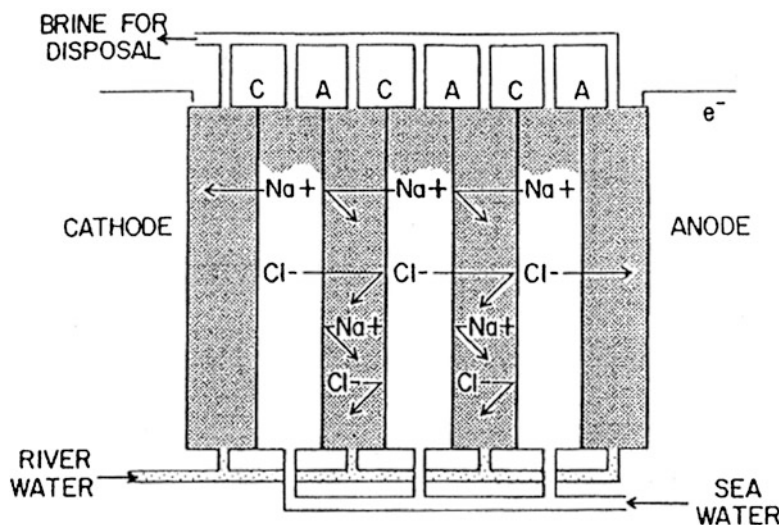
Fig. 1.16 The conversion of chemical potential into electrical energy by reverse electrodesalination
