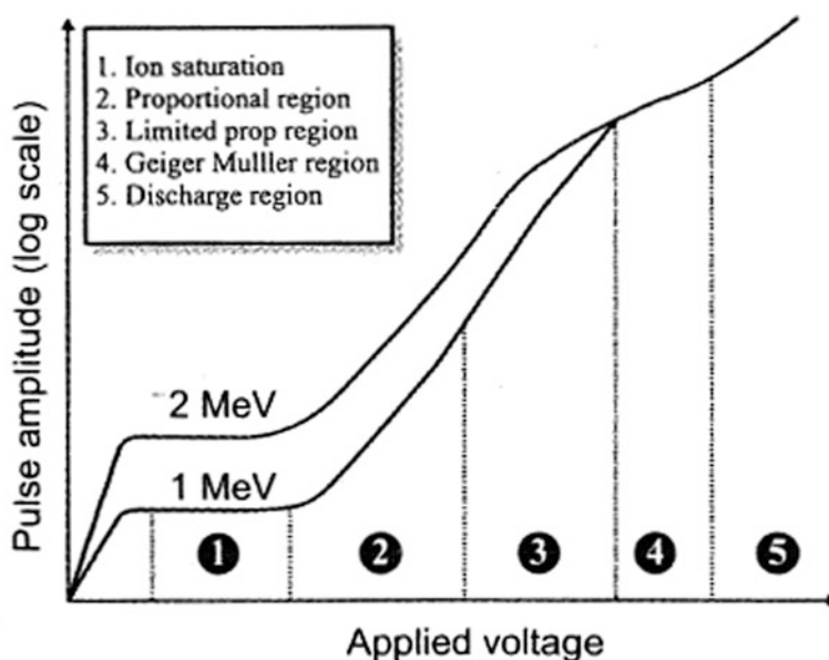
Fig. exp. 7.3 Variation of the charge induced at the anode with the applied voltage in an ionization counter
