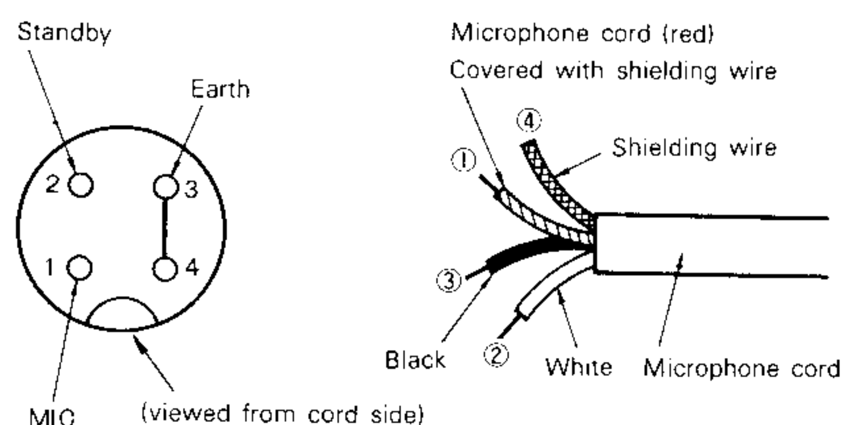
FIG. 24 CONNECTION OF MICROPHONE CONNECTOR
