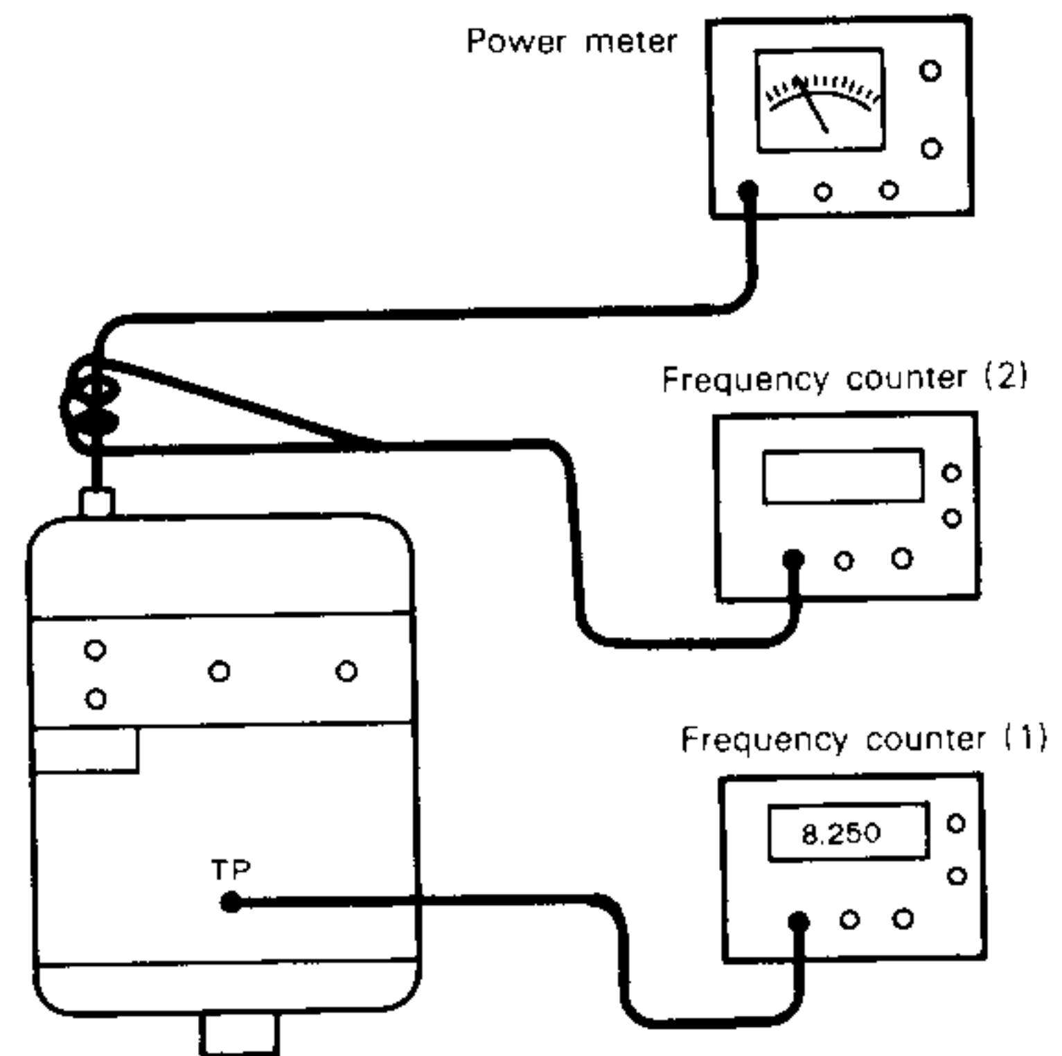
FIG. 19 FREQUENCY ADJUSTMENT
