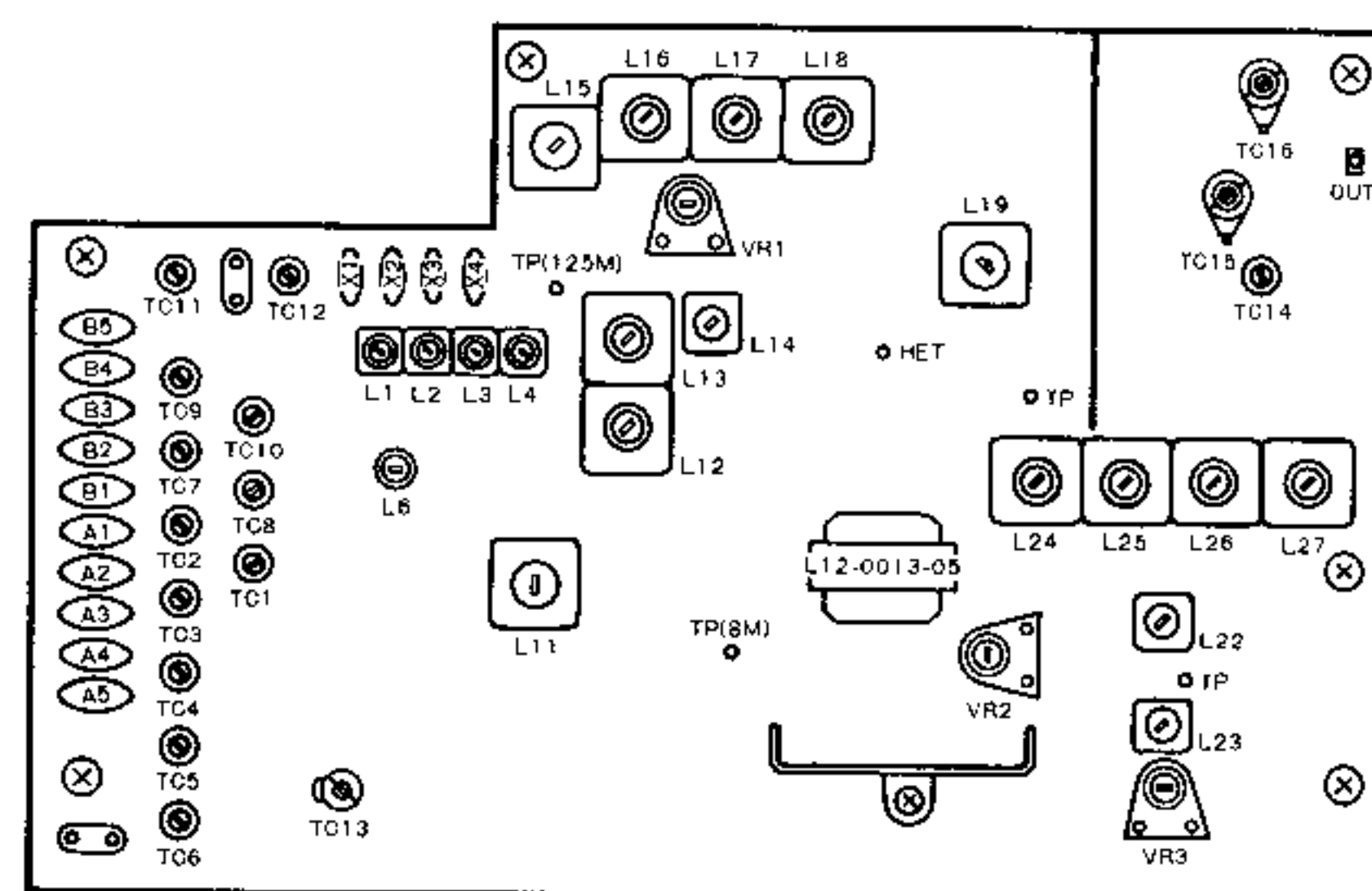
FIG. 2 SYNTHESIZER UNIT
