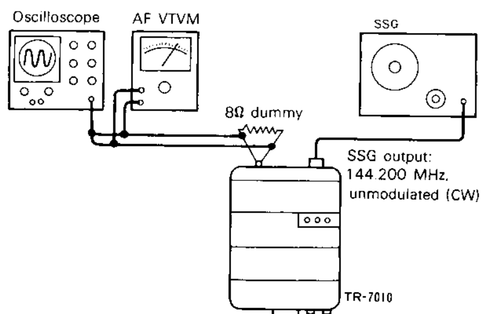
FIG. 16 RECEIVE SENSITIVITY ADJUSTMENT
