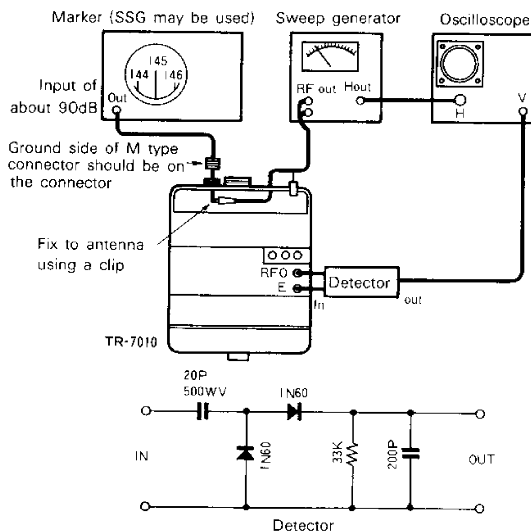
FIG. 12 HELICAL ADJUSTMENT
