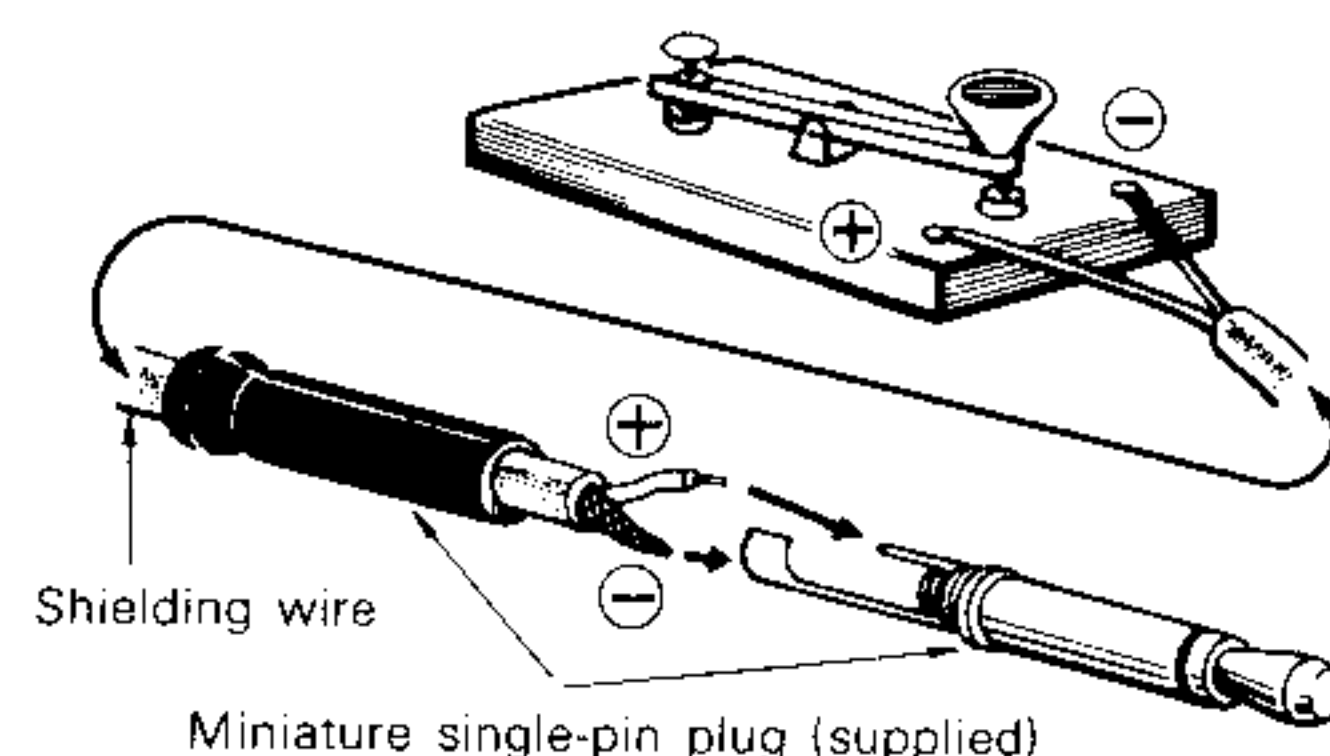
FIG. 22 KEY CONNECTION
