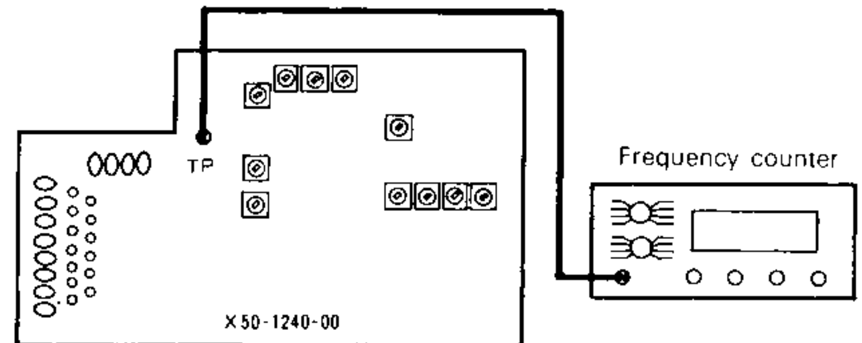
FIG. 4 41MHz OSCILLATION ADJUSTMENT
