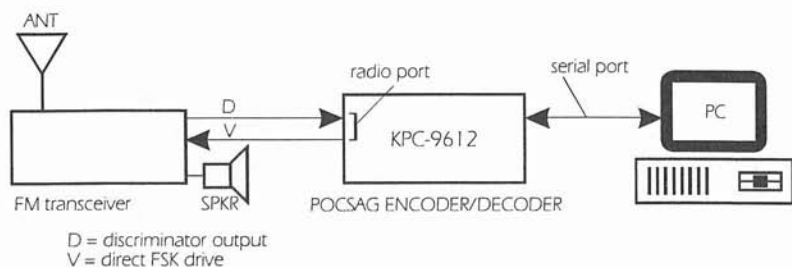
Figure 3-1: Monitor Station or Two-Way POCSAG Station
