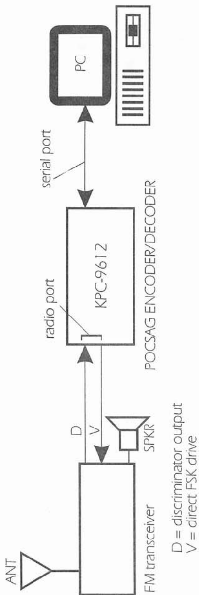
Figure 7-1: Paging Station: Transmit, Two-Way, or Monitor
