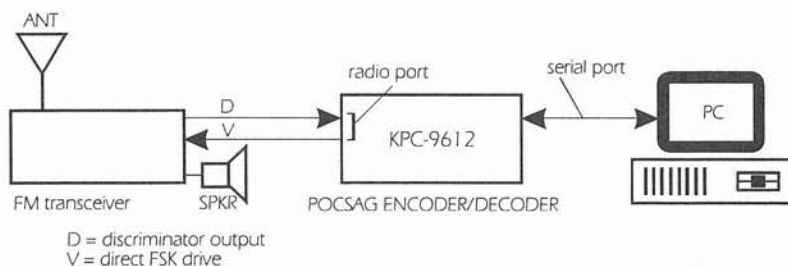
Figure 7-1: Paging Station: Transmit, Two-Way, or Monitor
