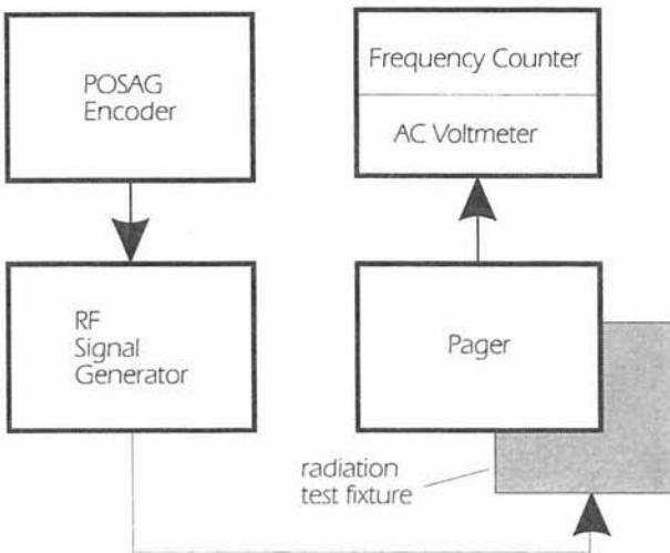
Figure 6-2: Pager Test Station
