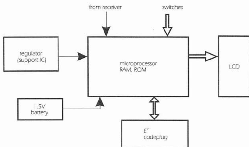
Figure 4-2: Pager Decoder Board
