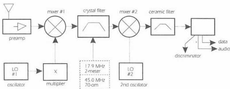
Figure 4-1: Pager Receiver
