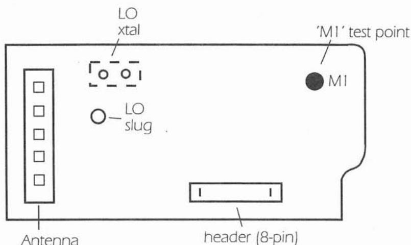
Figure 6-1: VHF Receiver Board AARD405X Series
