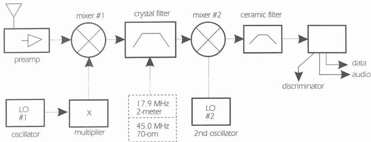
Figure 4-1: Pager Receiver
