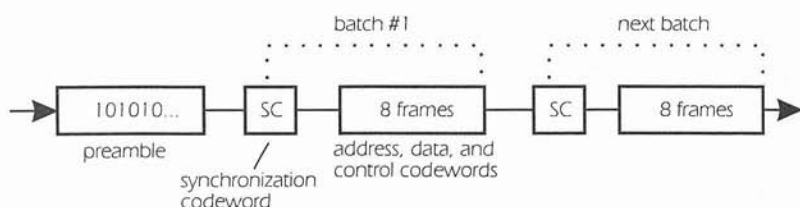
Figure 3-2: Page Signal Format
