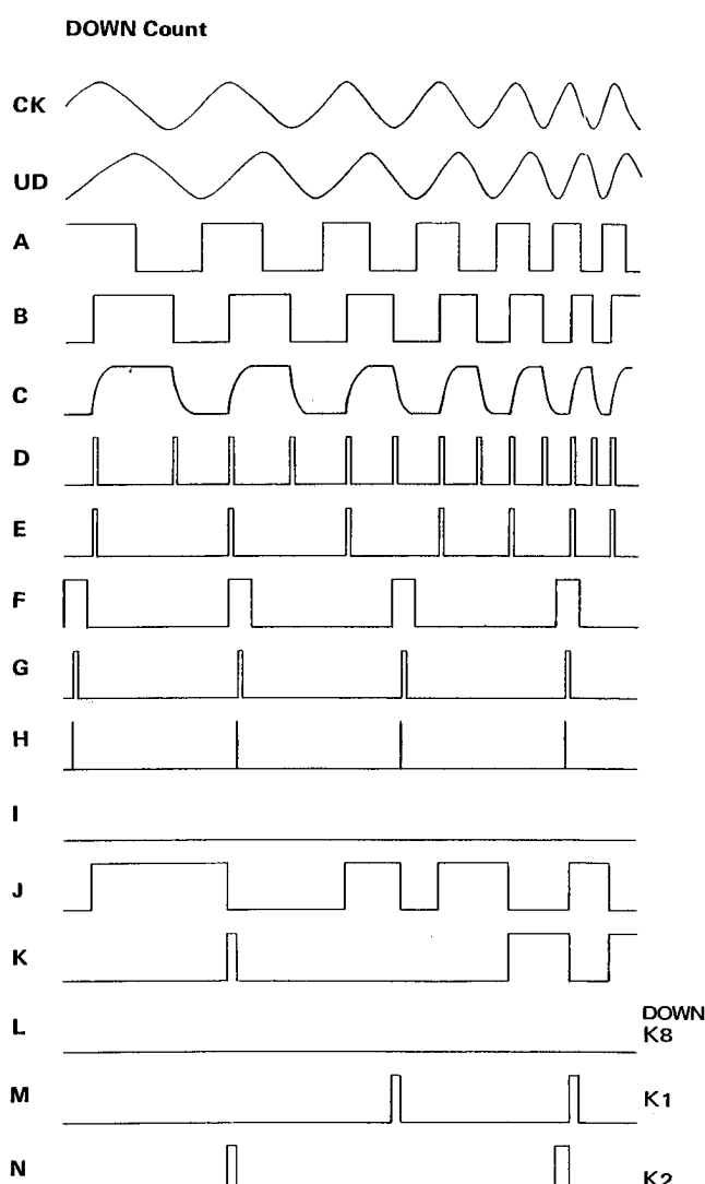
Timing Chart
