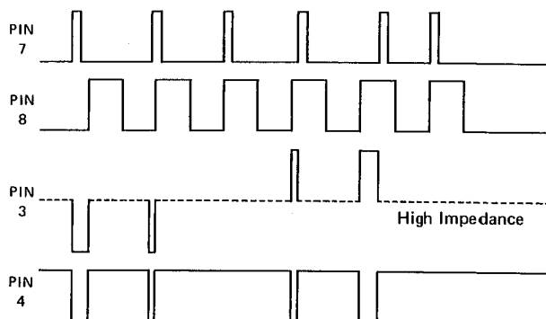
INPUT/OUTPUT WAVE FORMS OF PHASE DETECTOR IC2
