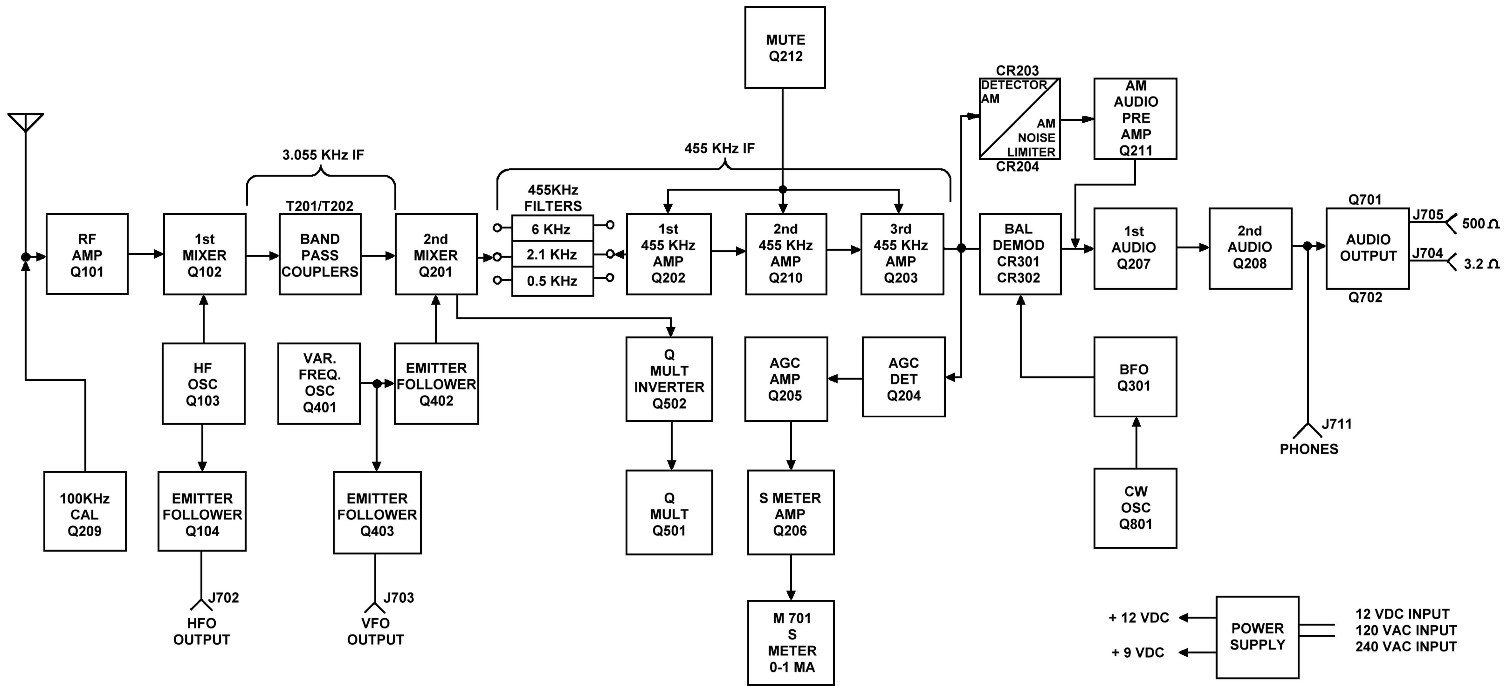
HAMMARLUND HQ-215 BLOCK DIAGRAM
