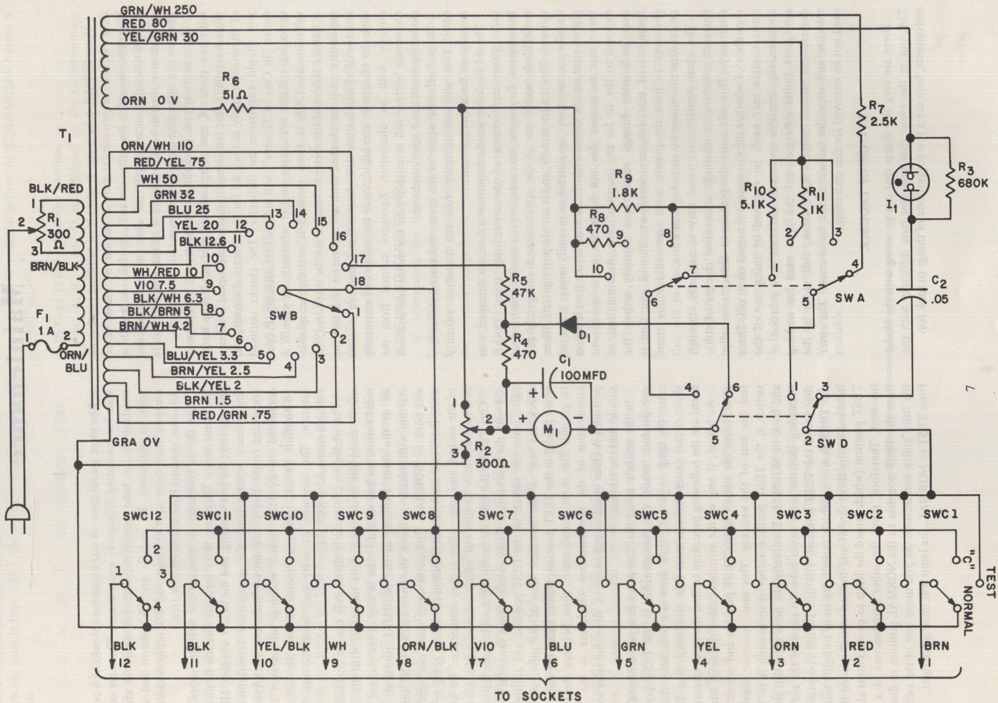
Schematic diagram of your CONAR Model 224 Tube Tester.
