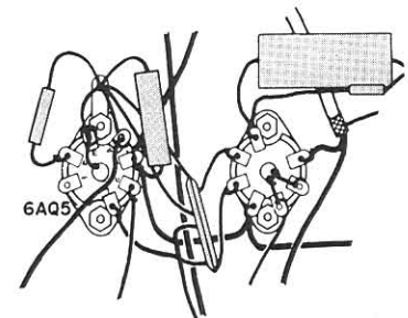
FIG. 4. First audio and audio output stages of a typical television receiver.
