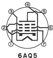
FIG. 5. Diagram of a 6AQ5 tube.
