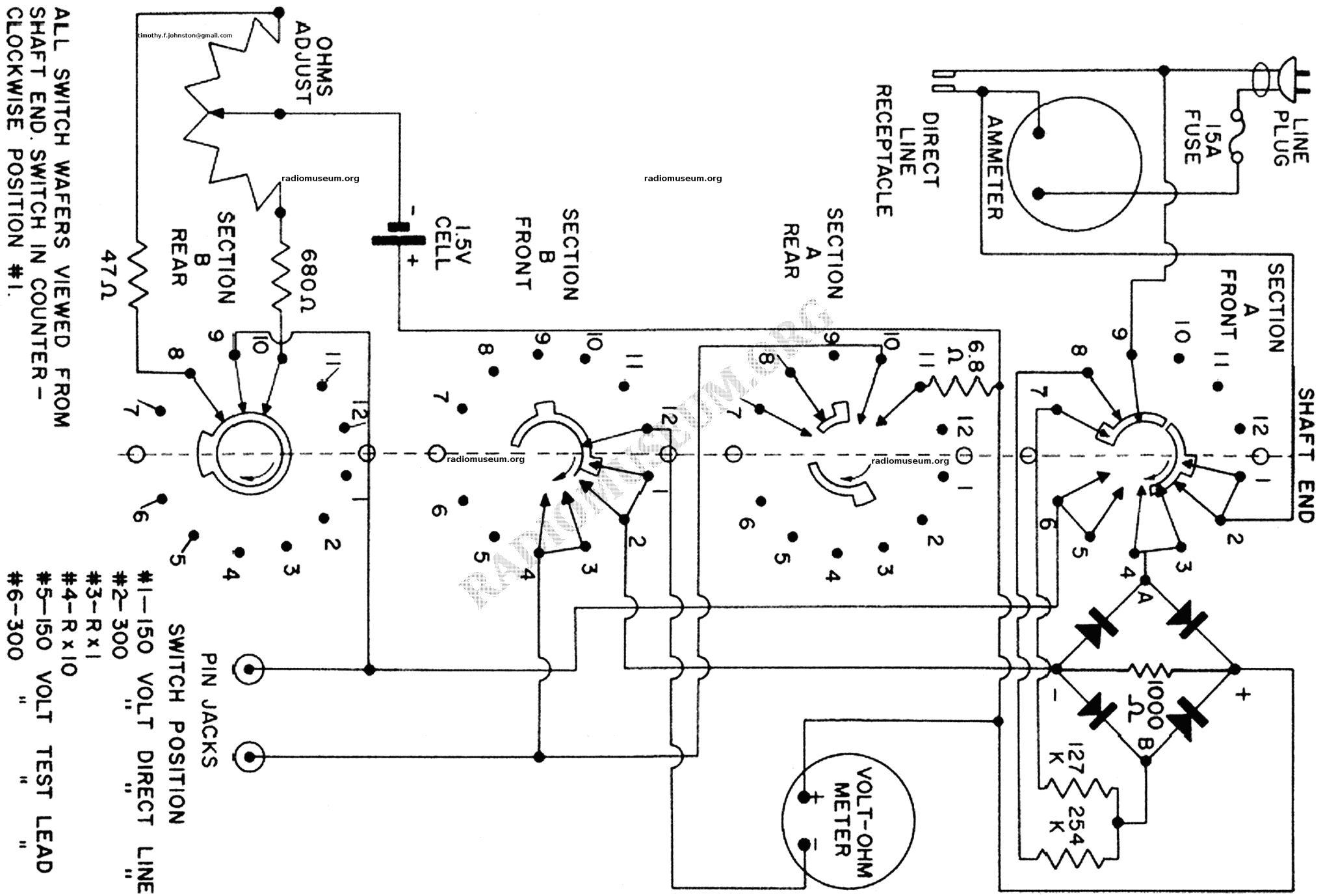
FIG. 7. Complete schematic diagram of Tester.
