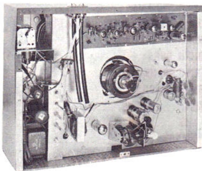
CONAR Custom 70 without rear cover, shield can and power cord
