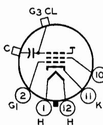
A ULTOR = G_3 + CL
