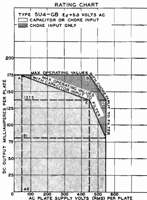
OPERATION CHARACTERISTICS FULL-WAVE CIRCUIT, CAPACITOR INPUT TO FILTER
