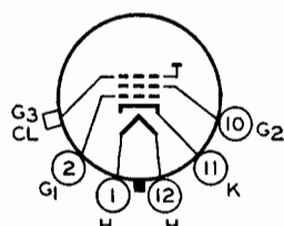
F ULTOR = G_3 + CL
