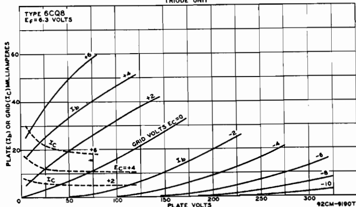
AVERAGE CHARACTERISTICS TRIODE UNIT
