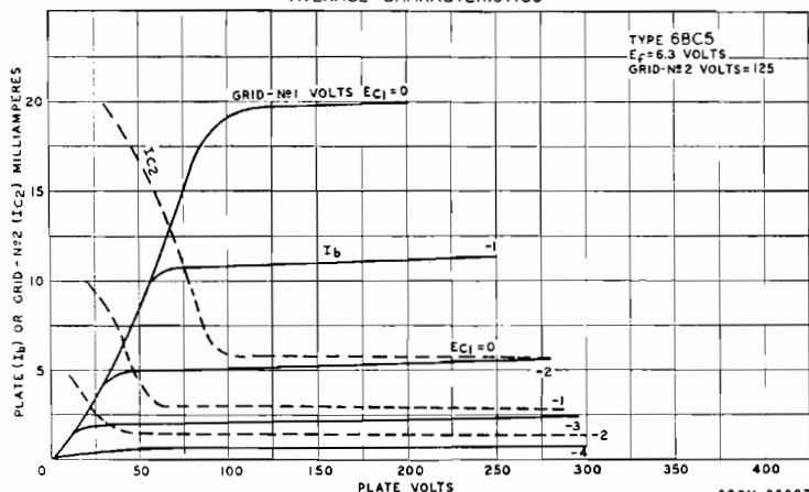
AVERAGE CHARACTERISTICS
