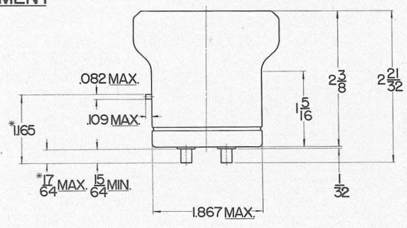
BASE NO. 500IB
