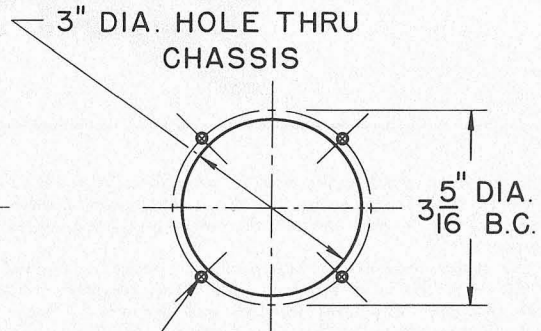
CHASSIS DRILLING
