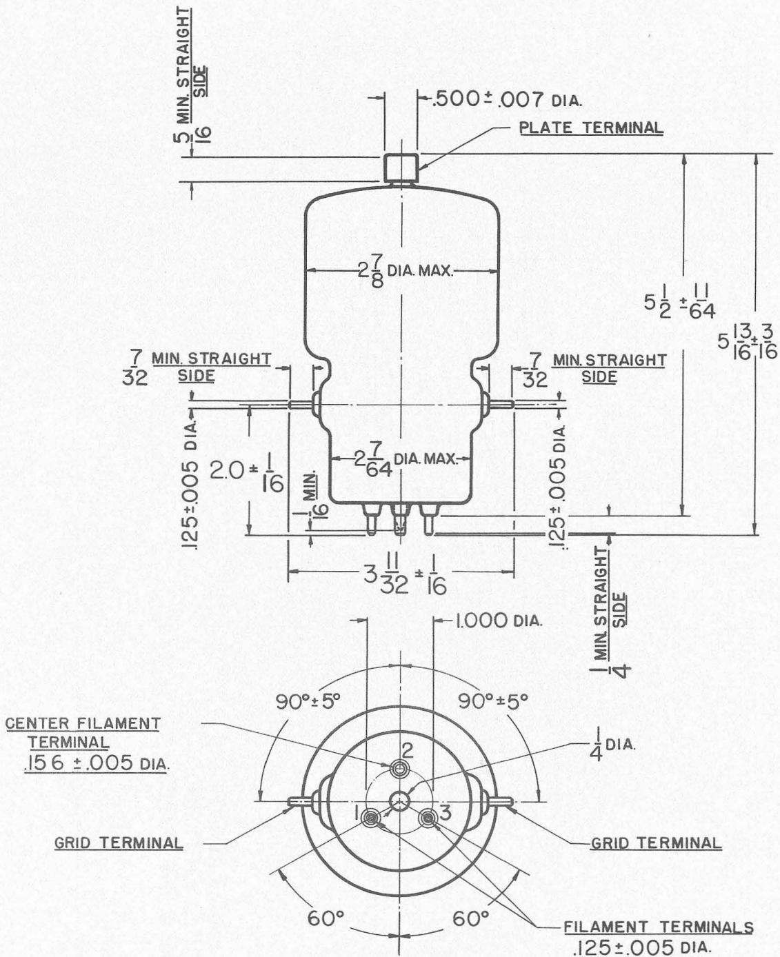
BOTTOM VIEW
