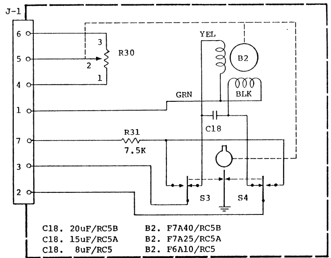
Figure 6-1 Rotor RC5, RC5A
