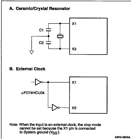
Figure 1. System Clock Configurations
