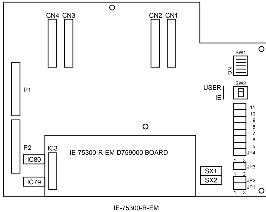
Figure 1-2. IE-75300-R-EM and Its Product Configuration (1/3)
