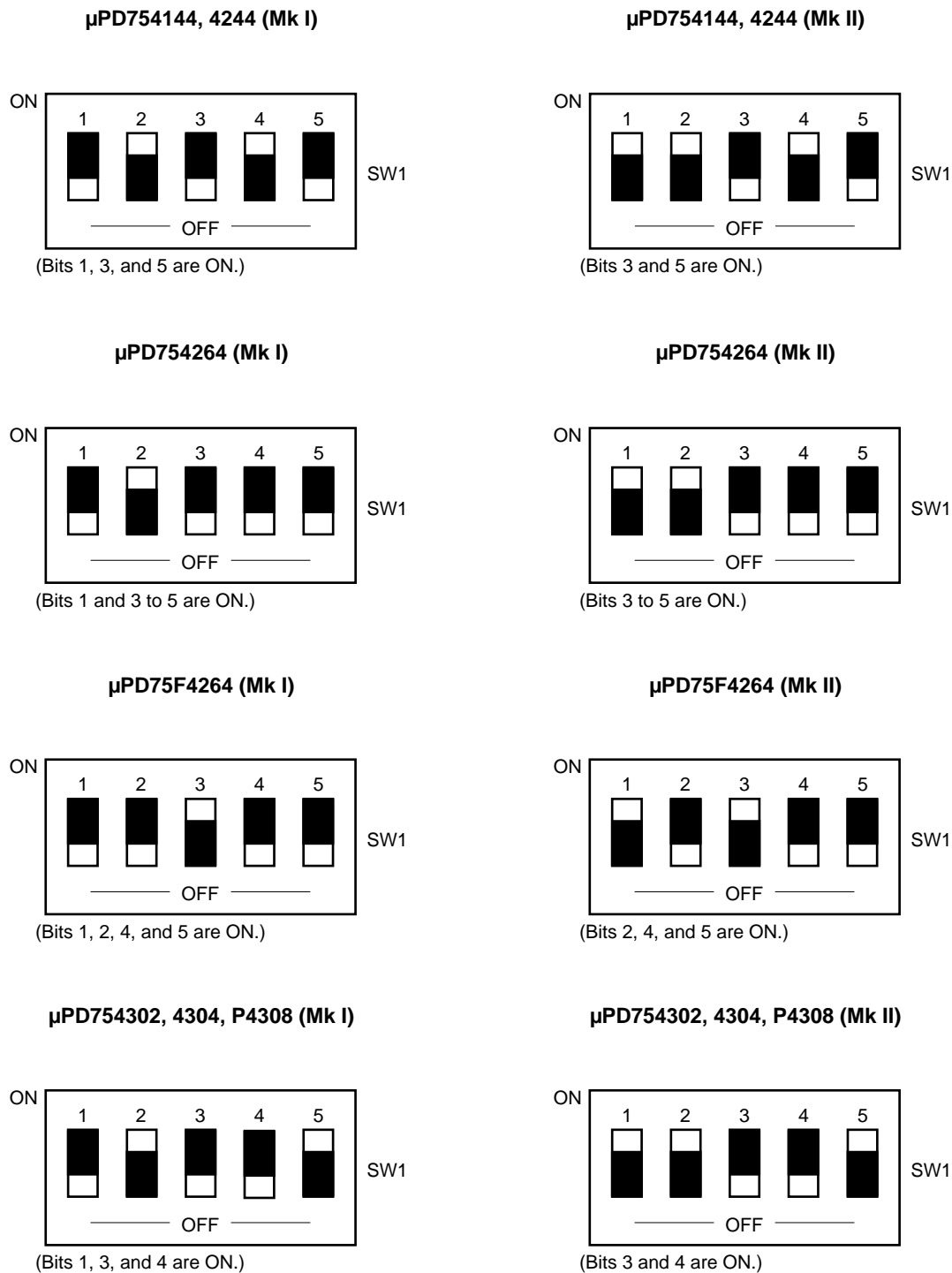
Figure 2-13. SW1 Setting (4/4)
