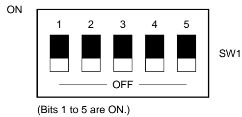
Figure 1-4. SW1 Setting (for shipment of IE-75300-R-EM)
