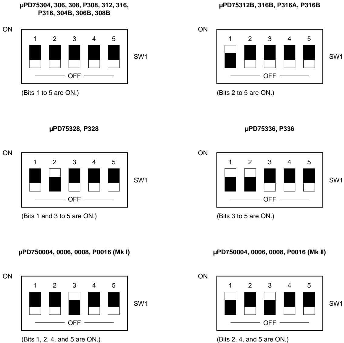
Figure 2-13. SW1 Setting (1/4)
