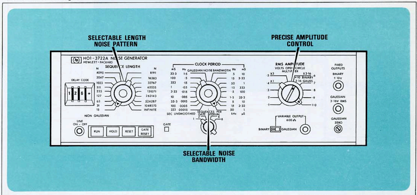
Figure A-1. Front panel of model H01-3722A noise generator
