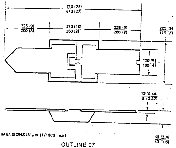
Figure 2. The dimensions of outline 07 are indicative of the small size of the beam lead package, resulting in little space needed in a circuit.
