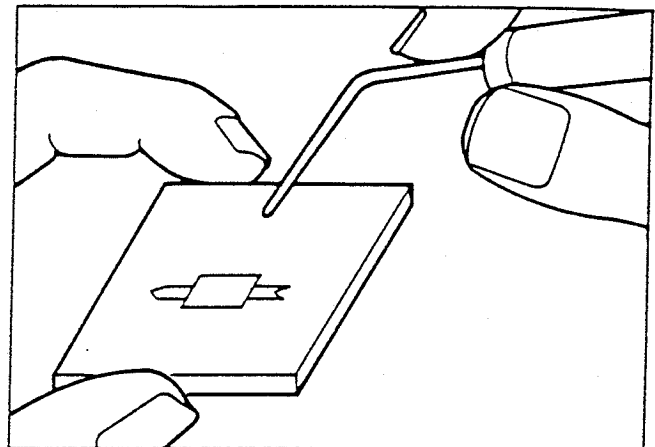
(d) A very efficient commercially available pick up tool has a teflon tip to which the device adheres.
