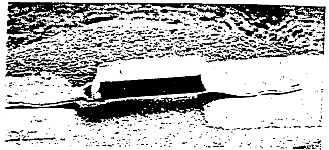
Figure 14. The HPND-4001 beam lead PIN diode bonded in package C-2 shown here is an example of a good bond. The beam leads are flat against the package contact metalization. The bond is centered on each lead with sufficient indentation.
