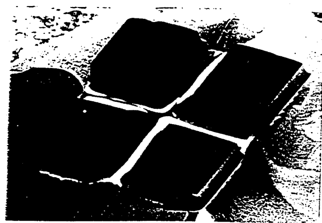
Figure 19. This is another example of a poorly executed bond. The quad is twisted so badly that the bottom lead has separated.
