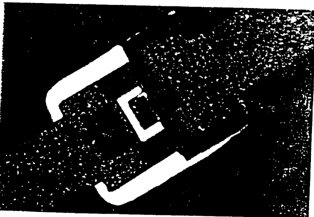
Figure 1. The HPND-4001 beam lead PIN diode in outline 07 shown here provides low capacitance of 0.07 pF and less than 0.1 nH inductance to allow the achievement of maximum isolation and minimum insertion loss at high frequencies.
