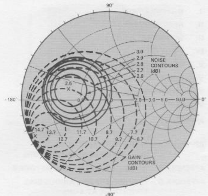
Figure 2. Impedance Coordinates.
