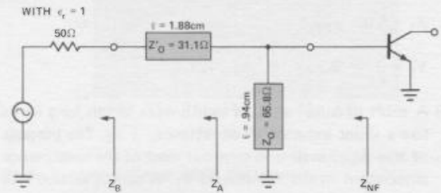
Figure 4. Impedance Coordinates.
