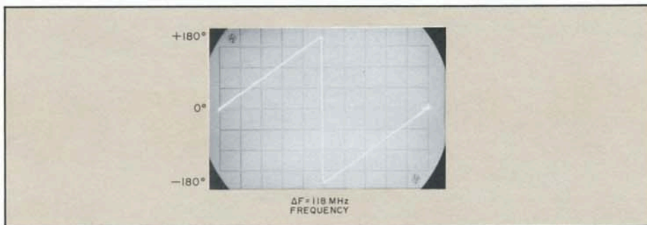
Figure 5. TWT amplifier measures total group delay. The sweep oscillator bandwidth is adjusted for 360^\circ of linear phase shift. Group delay then reduces to the equation: t_D = 1/\Delta f . Here \Delta f = 118 MHz, indicating 8.5 nanoseconds of delay.
