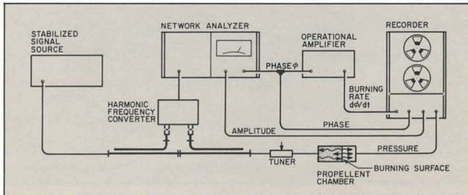
Figure 9. Block diagram showing system for measuring burning rate of a solid propellant using the Doppler shift principle.
