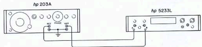
Figure 10. Phase Dial Calibration With Time Interval Counter.
