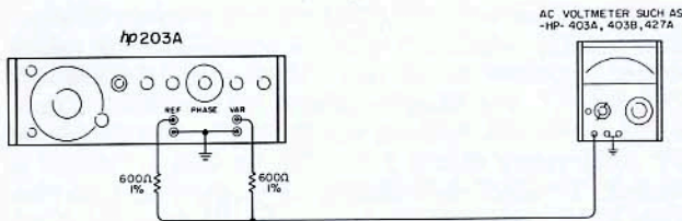
Figure 8. Setup For Measuring 180° Phase Shift
