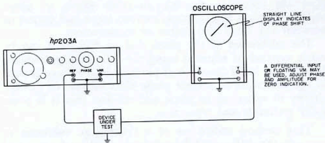
Figure 3. Setup to Measure Phase Shift of Components
