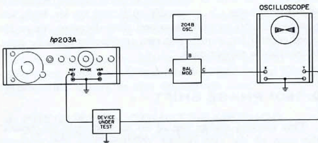
Figure 4. Setup to Measure Phase Shift Using Bow Tie Method
