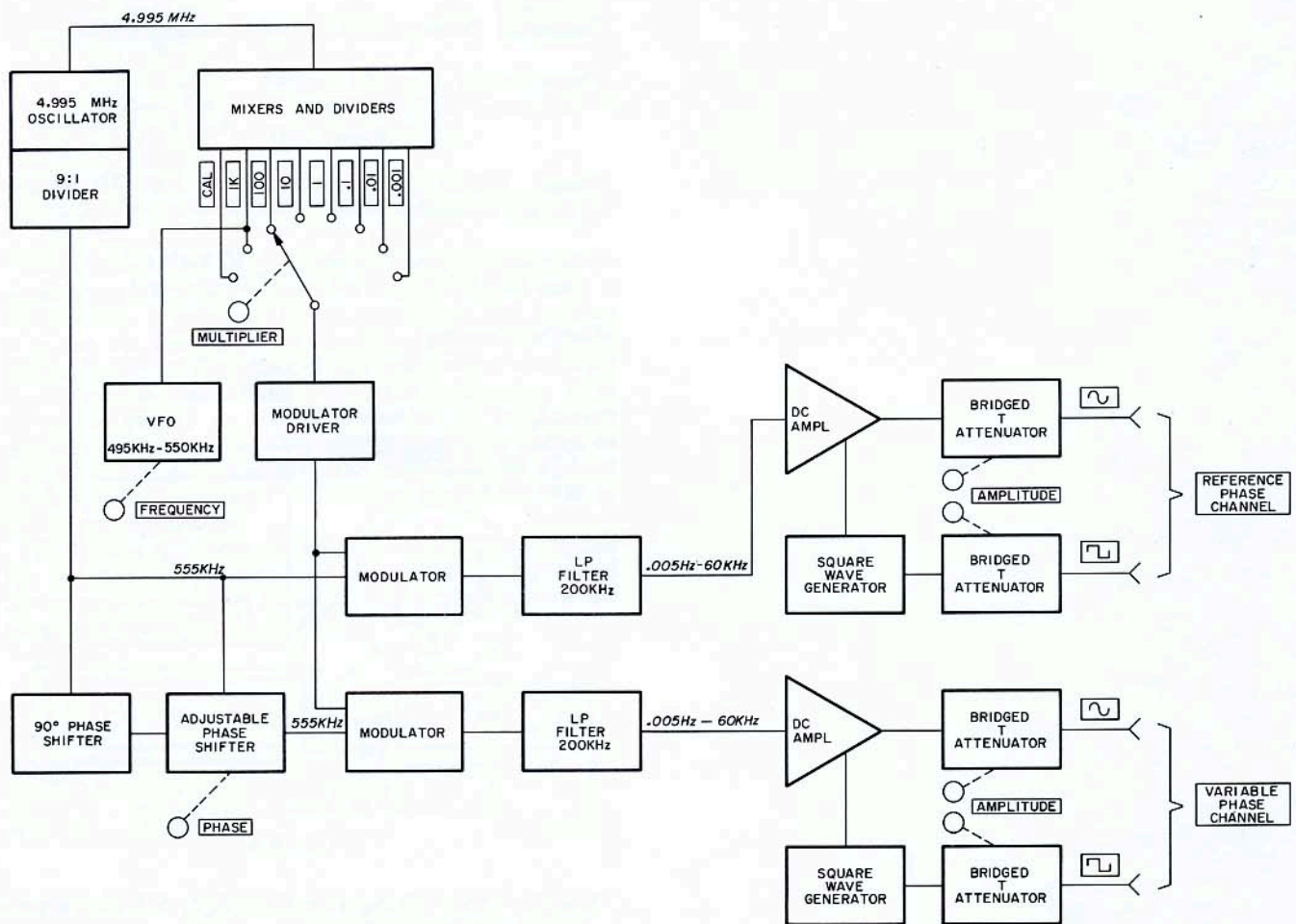
Figure 1. 203A Block Diagram
