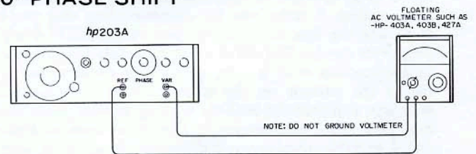
Figure 7. Setup For Calibrating 0° Phase Shift
