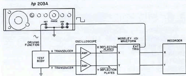
Figure 12 Hysteresis Curve Plotting.
