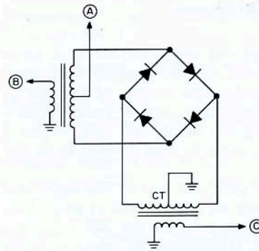
Figure 6. Details of Balanced Modulator
