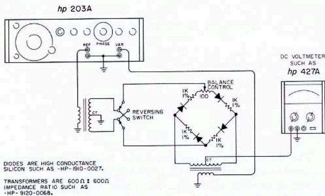
Figure 9. Setup For Calibrating 90° and 270° Phase Shift
