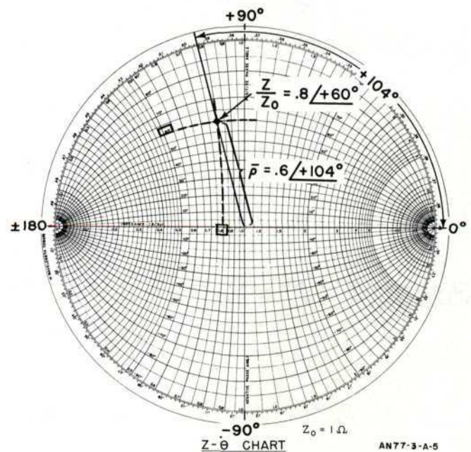
Figure 6. Z - \theta Chart
