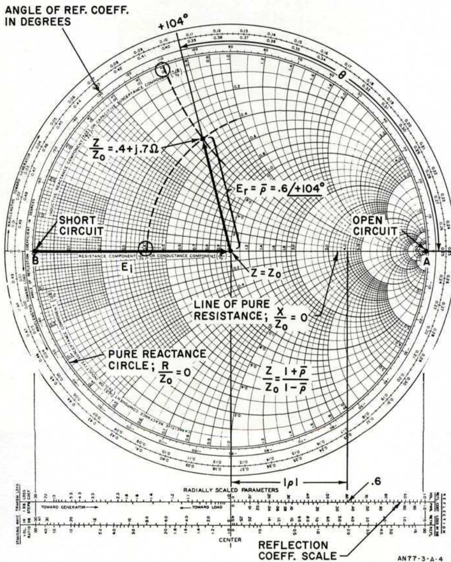
Figure 5. Impedance & Reflection Coefficient Relationships on Smith Chart
