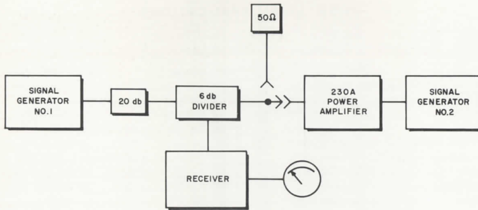
Figure 2. Connections for Desensitization Test
