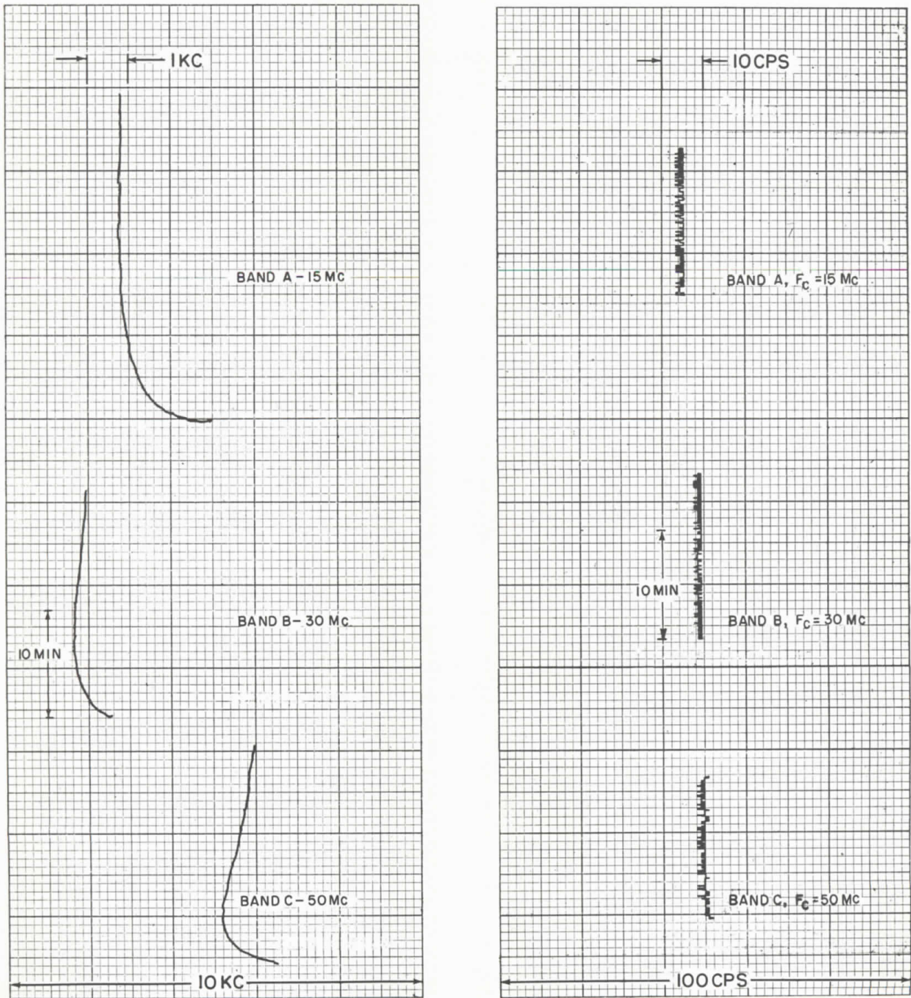
Figure 15a. Strip chart recordings compare frequency stability of hp 608F on three bands for unlocked (left), and phase-locked (right) operation. Note different span calibrations for frequency; span sensitivity increase of 100 in right hand recording magnifies \pm 1 count ambiguity of counter causing fine grain variations. Also note time to restabilize after band switching when unlocked.
