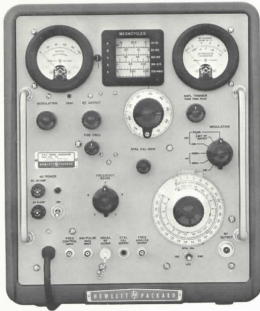
Figure 3. HP 608F Signal Generator provides up to 0.5 volt from 10 Mc to 455 Mc with the ability to be phase locked to the HP 8708A Synchronizer. Drastic reduction of drift and microphonics with phase lock eliminates a large source of error when testing high slope or narrow-band circuits. Linear FM and PM is also possible when phase locked, opening new areas of application.
