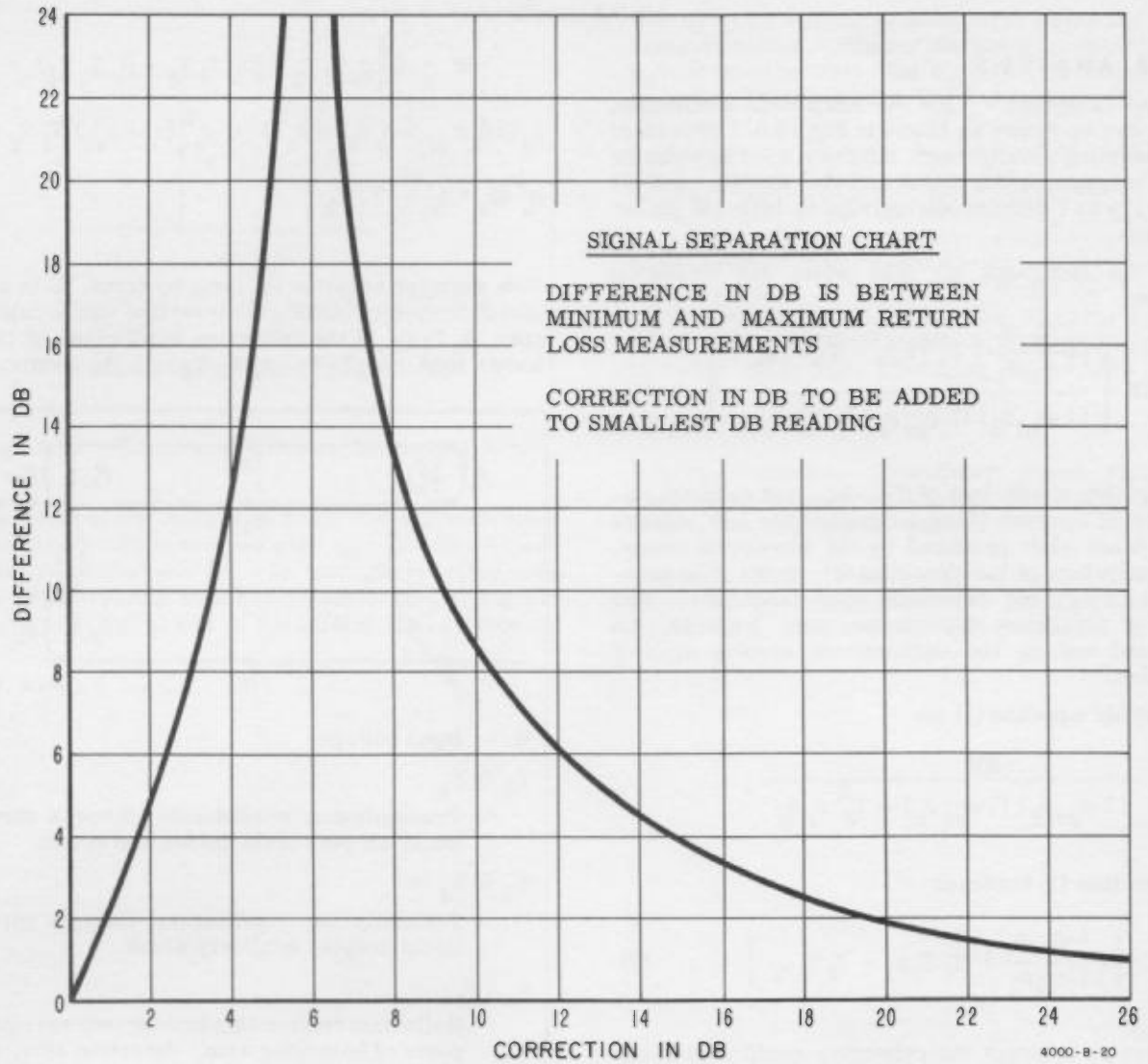
Figure 9. Chart for separating two signals when their sum and difference are known
