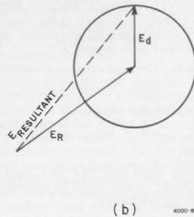
Figure 1. (a) Leveled Coaxial Reflectometer (b) Vector Diagram of Voltage Components Comprising Signal at Port 3 of Coaxial Reflectometer
