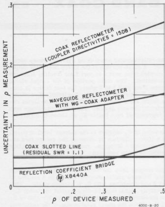
Figure 2. Uncertainty of various reflection coefficient ( \rho ) measuring techniques vs actual \rho of device in test. Curves are typical for coaxial systems at X-band frequencies.
