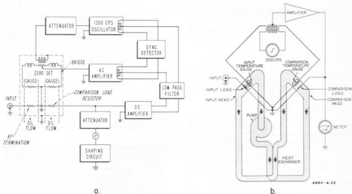
Figure 2-21. Block diagram (a) and oil flow diagram (b) of hp 434A Calorimetric Power Meter.
