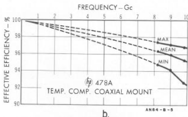
Figure 2-16. Typical efficiency data on (a) HP 477B coaxial thermistor mounts and (b) HP 478A temperature compensated coax mounts. Solid lines indicate data with NBS traceability. Recent NBS calibrations indicate dashed line interpolation is valid at 3 Gc also. Actual data is now stamped on each hp 478A compensated mount for highest accuracy.
