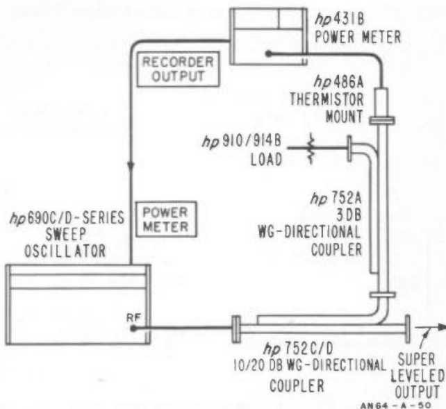
Figure 4-3. Super-leveled waveguide system.
