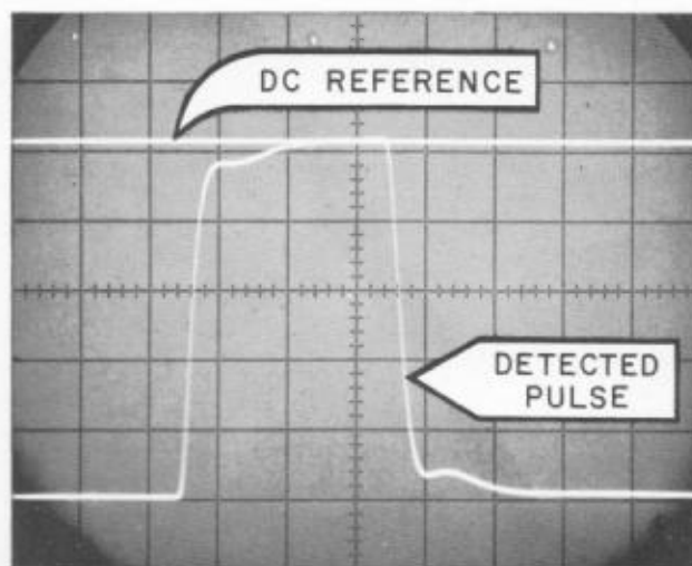
Figure 3-18. Oscilloscope display of Boonton 8900B video output enables selective positioning of DC reference on RF pulse envelope. Meter on 8900B then reads reference directly in peak pulse power.
