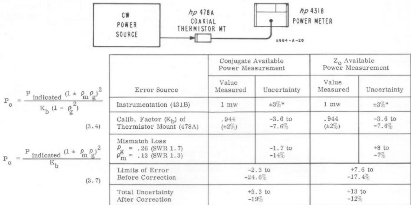
Figure 3-2a. Basic system for coaxial power measurements of 10 μw to 10 mw full scale, 10 Mc - 10 Gc. Chart lists sources of error and examples of their effects on the measurement. Equations show relationship of indicated power to conjugate available power (P c ) and Z o available power (P o ).
