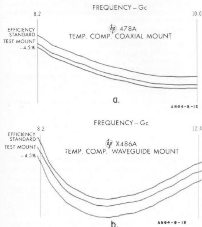
Figure 3-10. Swept frequency efficiency plots of (a) HP 478A coax thermistor mount (b) HP X486A waveguide mount, compared to a standard mount with system in Figure 3-9. Note absence of efficiency "holes" sometimes found in defective mounts.
