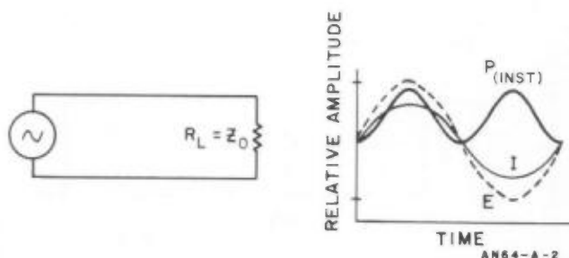
Figure 1-2. Instantaneous power in load resistor R_L varies at a rate twice the applied generator frequency.
