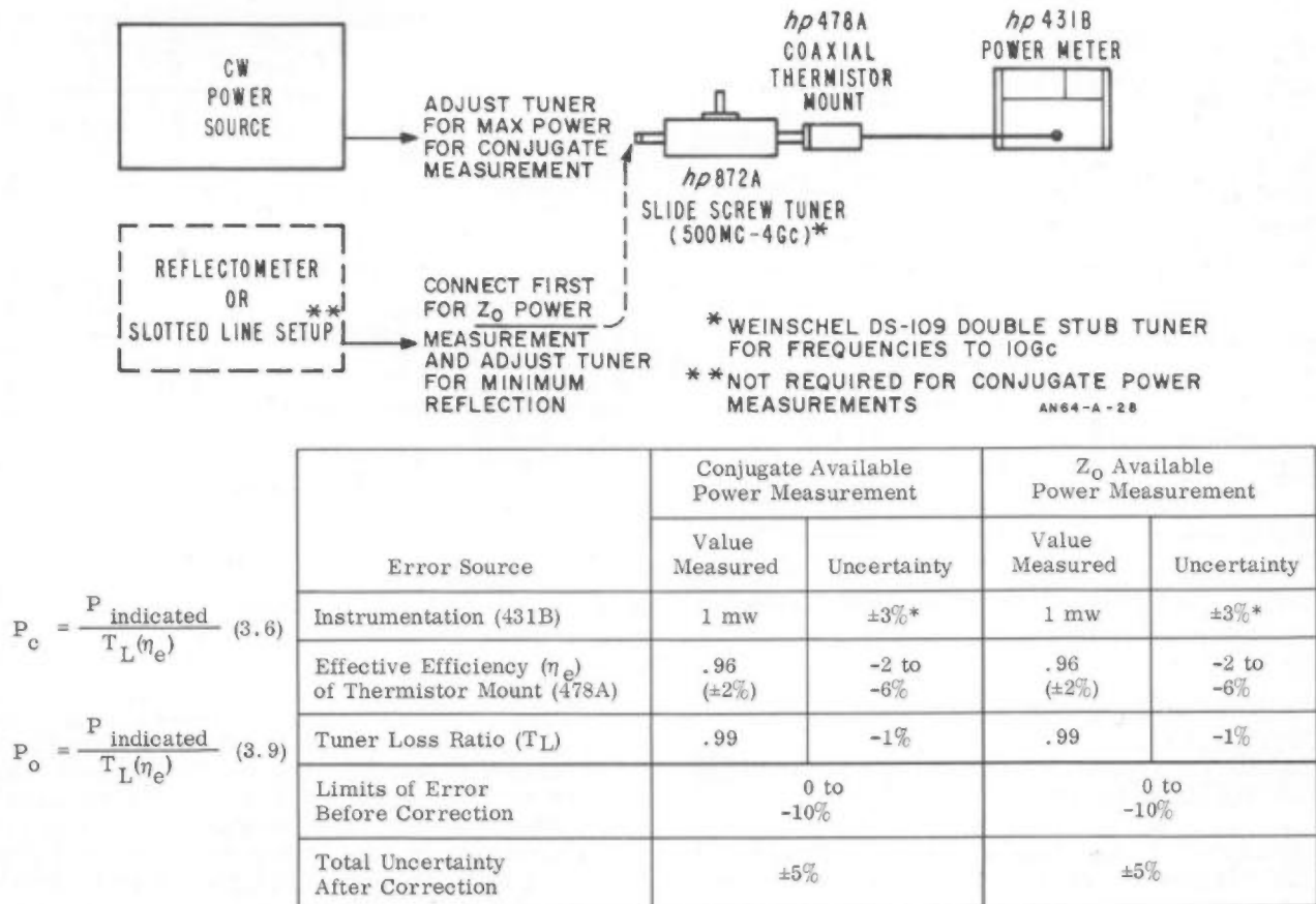
Figure 3-2a. Basic system for coaxial power measurements of 10 μw to 10 mw full scale, 10 Mc - 10 Gc. Chart lists sources of error and examples of their effects on the measurement. Equations show relationship of indicated power to conjugate available power (P c ) and Z o available power (P o ).
