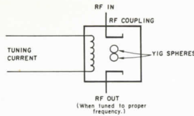
Figure 1. YIG Tuning Circuit
