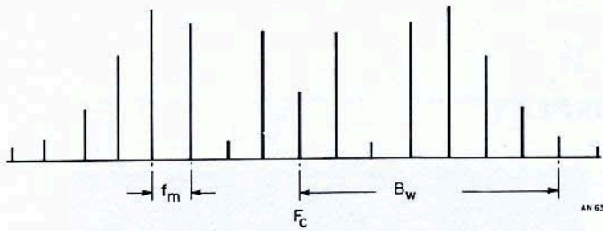
Figure 5. Amplitude Spectrum of Single Tone Frequency Modulation
