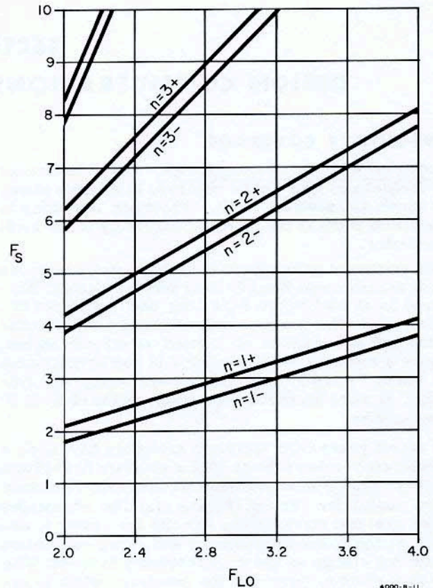
Figure 12b. Analyzer Tuning Curves for F_{if} = \frac{F_{LO}(\text{min})}{10} F_s = nF_{LO} \pm 200 \text{ mc}
