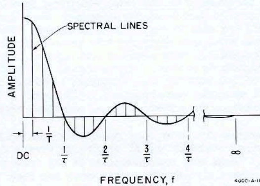
Figure 7. Spectrum of a perfectly rectangular pulse. Amplitudes and phases of an infinite number of harmonics are plotted resulting in smooth envelope as shown.
