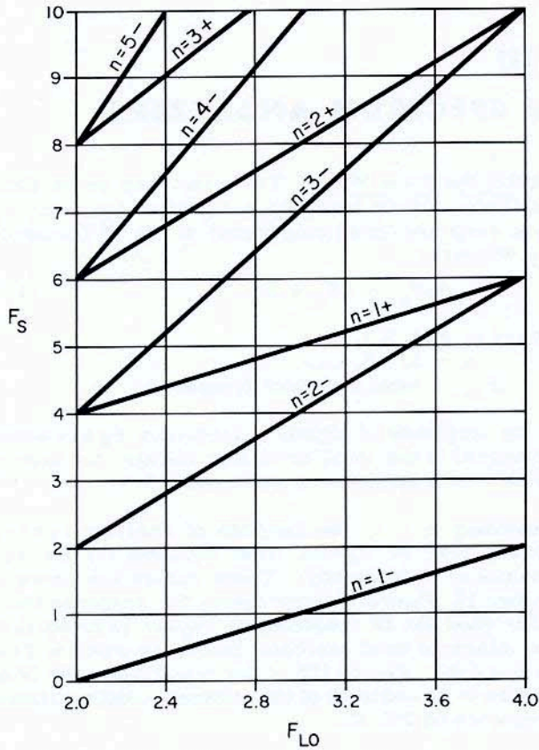
Figure 12a. Analyzer Tuning Curves for F_{if} = F_{LO}(\text{min}) F_s = nF_{LO} \pm 2 \text{ gc}
