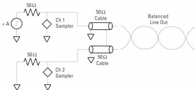
Figure 33. Differential TDR
