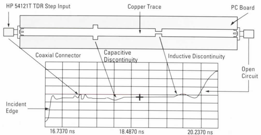
Figure 7. Typical performance characteristics
