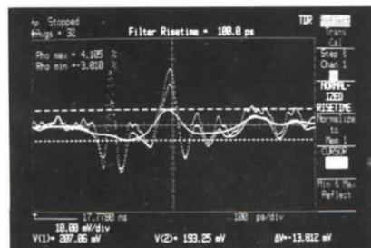
Figure 28. Hybrid measurement
