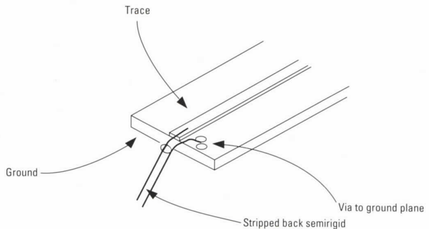
Figure 15. Semirigid cable launched onto trace and via hole
