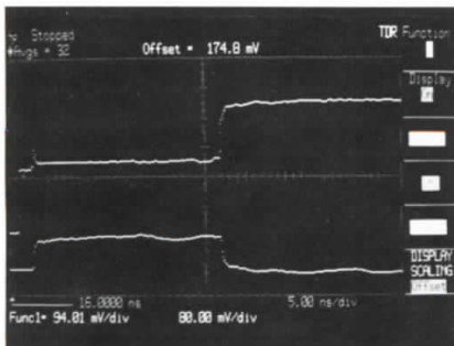
Figure 36. Twisted pair measurement
