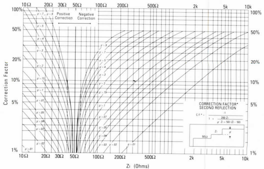
Figure 37. Second reflection correction factor
