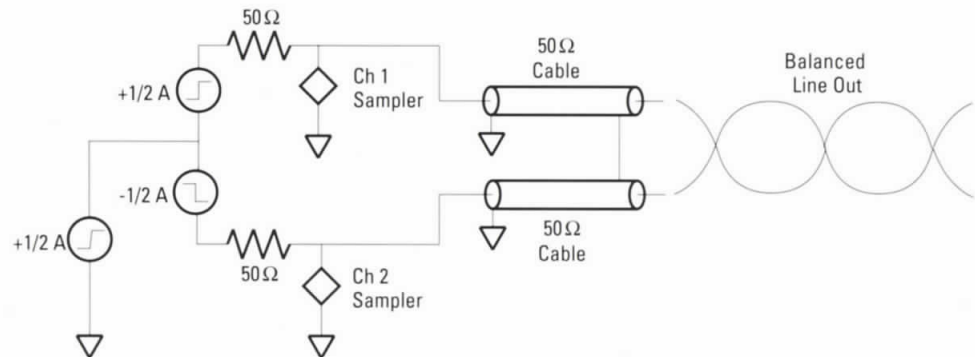
Figure 34. Differential TDR
