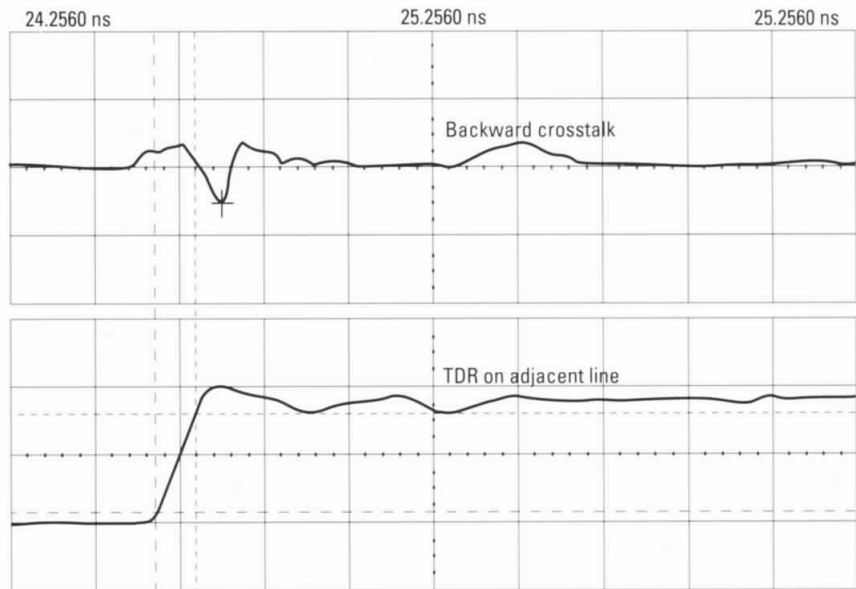
Figure 23. PC Board microstrip trace crosstalk
