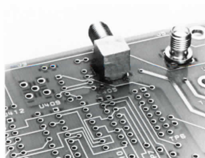
Figure 20. SMA 90° Launcher
