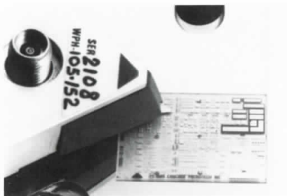
Figure 26. 50 \Omega probe tip to hybrid
