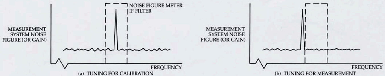
Figure 2.2 If the measurement system has noise figure or gain discontinuities, non-repeatable tuning between (a) calibration and (b) measurement can cause errors when correcting for second stage contribution.
