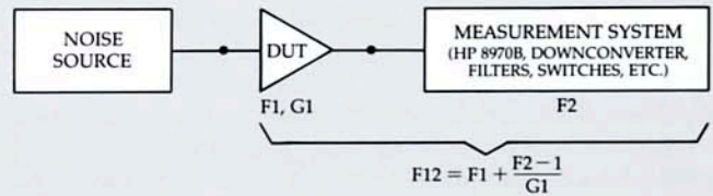
Figure 3.1 Typical noise figure measurement setup. Device and measurement system noise figures combine according to the cascade gain equation.
