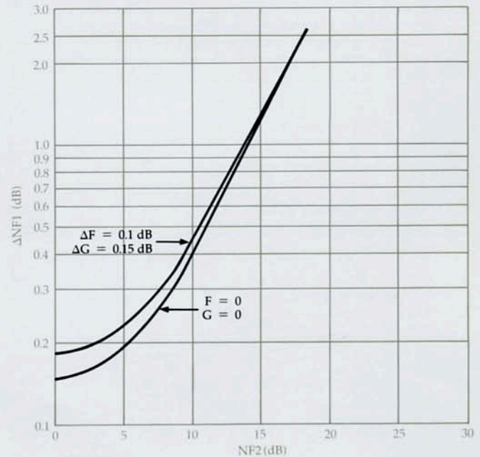
Figure 4.5 Comparison of effect of normal and zero instrumentation uncertainty on overall uncertainty.
