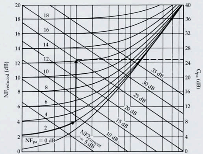
Figure 5.3 Graph to calculate preamp noise figure and gain. (Procedure for use is given in text.) Example shown: To reduce NF_{2\_current} (25 dB) to NF_{2\_reduced} (4 dB), a 2 dB noise figure, 25 dB gain preamplifier is needed.
