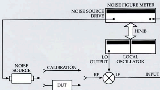
Figure 2.3 Microwave noise figure measurement set-up (double-sideband measurement).
