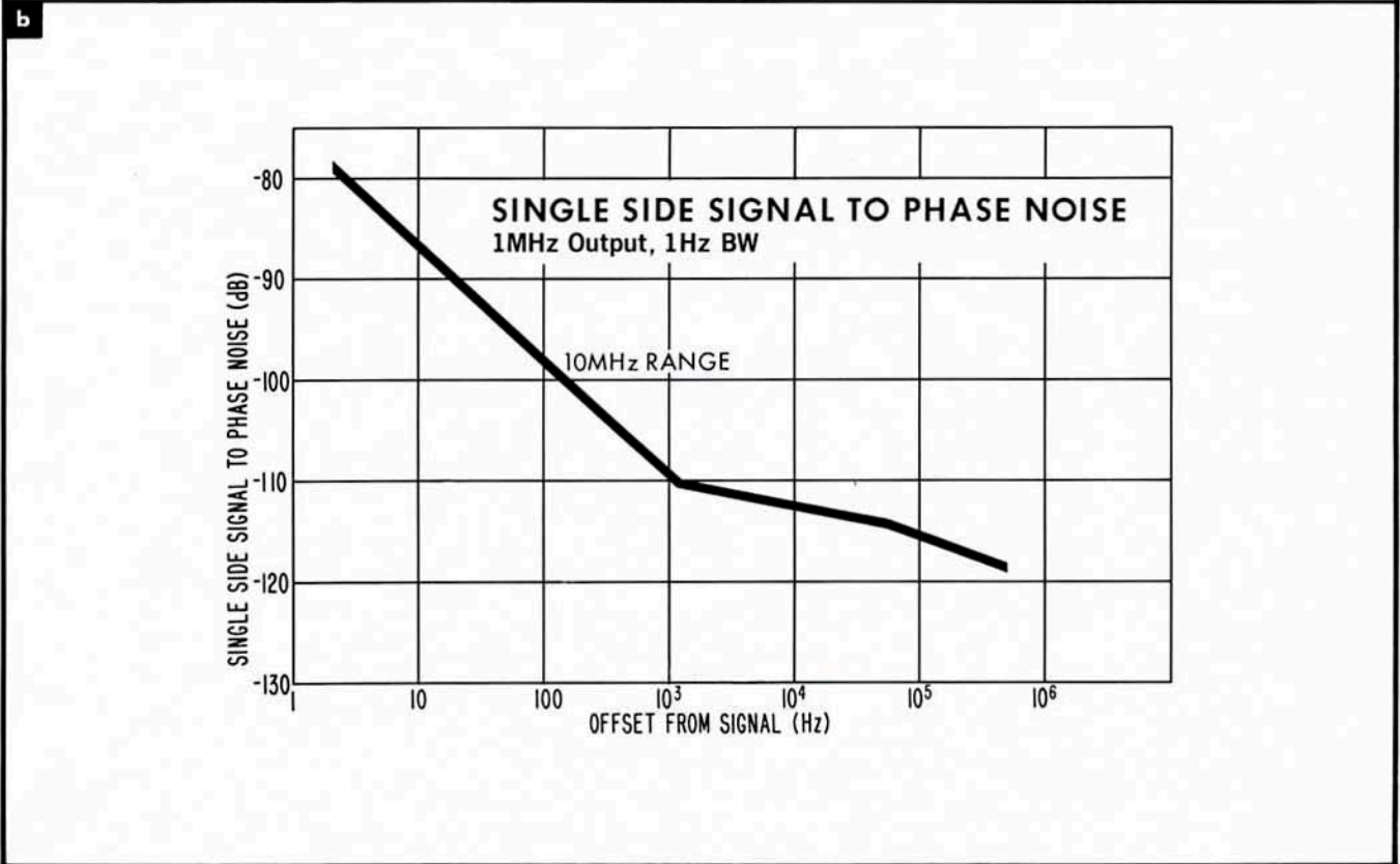
Figure 3-6. 5103A Frequency Synthesizer Phase Noise Plots
