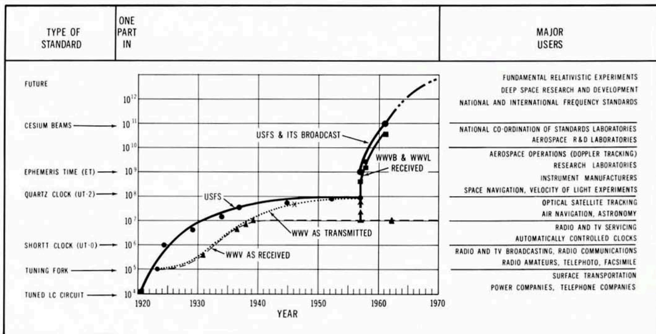
Figure II-1. Improvements in the precision of the U.S. Frequency Standard (USFS) and its dissemination.
