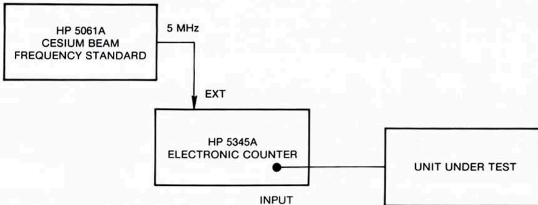
Figure 3-3. Direct Frequency Comparison with a Counter
