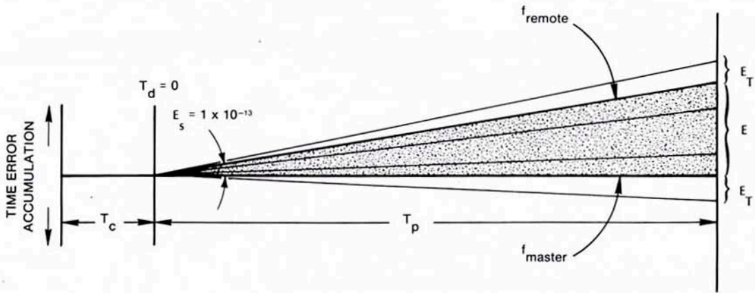
Figure 2-7. Comparison of Two Clocks
