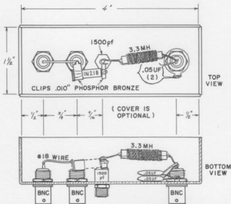
Figure 4. Construction Details of Crystal Mixer and Low Pass Filter
