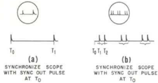
Figure 6. Sweep Calibration
