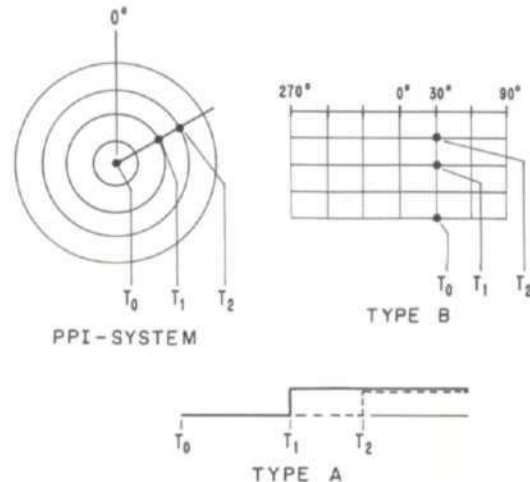
Figure 7. Radar System Calibration
