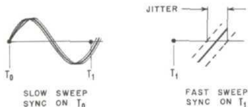
Figure 8. Jitter Measurement
