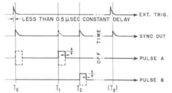
Figure 2. Time Plan, 219B Plug-In Unit
