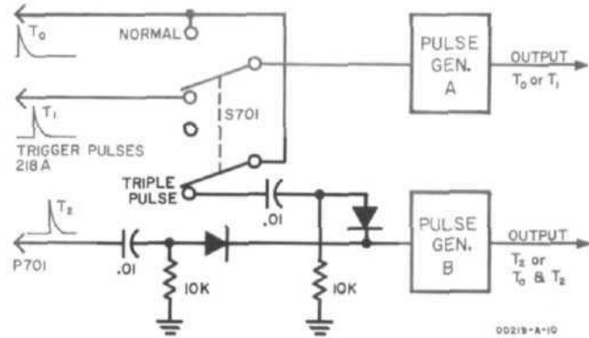
Figure 10. Triple Pulse Generator
