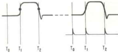
Figure 4. Measuring Waveforms
