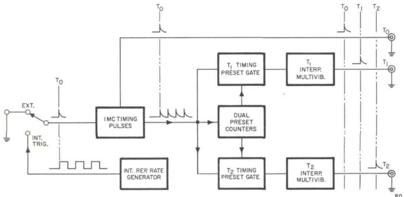
Figure 1. Block Diagram, Model 218A
