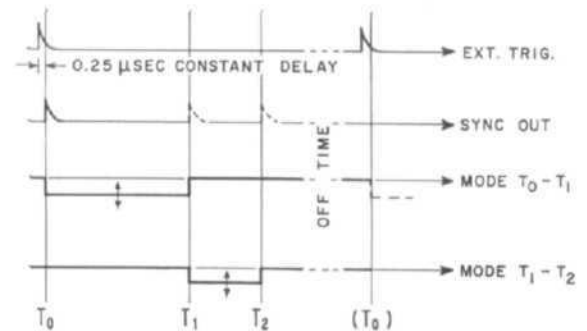
Figure 3. Time Plan, 219C Plug-In Unit
