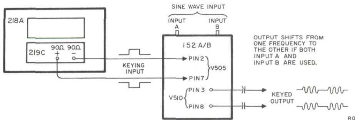
Figure 9. Using the 218A/219C with the 152A/B Oscilloscope Plug-In to Provide Pulse Bursts or Frequency Shift Keying
