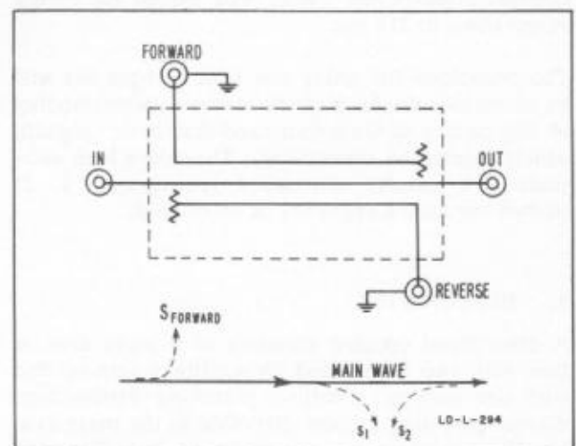
Figure 3. Schematic Diagram of Dual Directional Coupler
