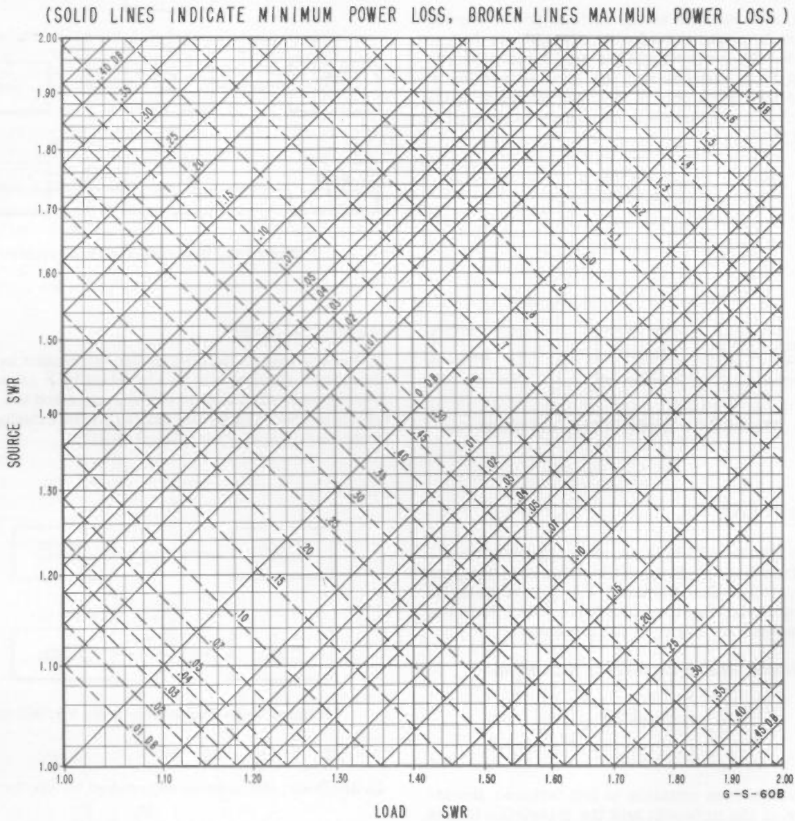
Figure 3-4. Mismatch-Loss Curves
