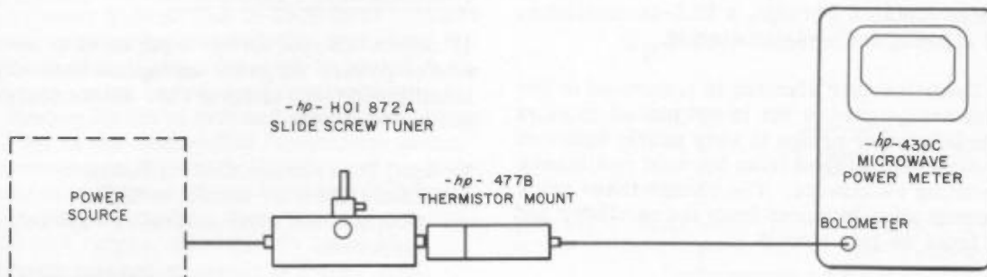
Figure 5-3. Power Measurements in Coax Systems
