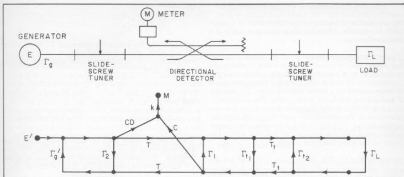
Figure 4. Single-Coupler Reflectometer
