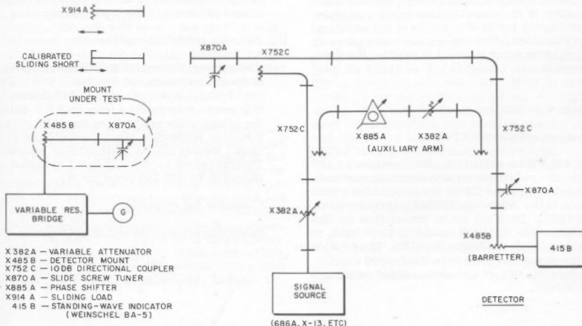
Figure 1 - Circuit Diagram
