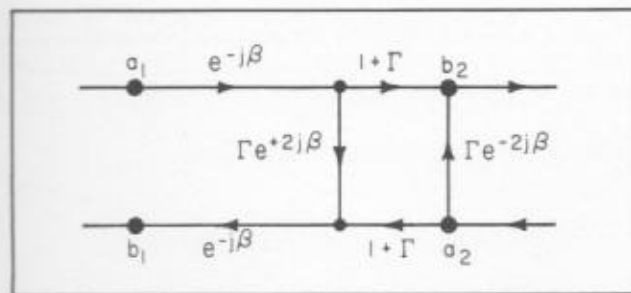
Figure 6 (b) - Equivalent Discontinuity Referred to the Other Port
