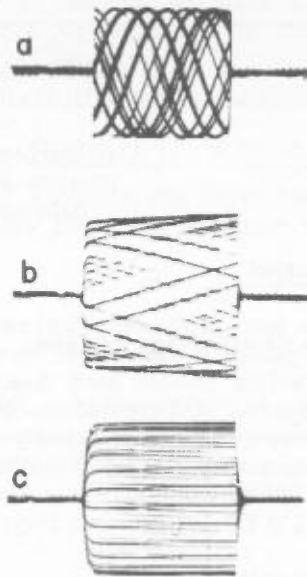
Fig. 3. Pulse Presentation for difference frequencies of (a) one, (b) one-tenth, and (c) one one-hundredth cycle-per-pulse-width
