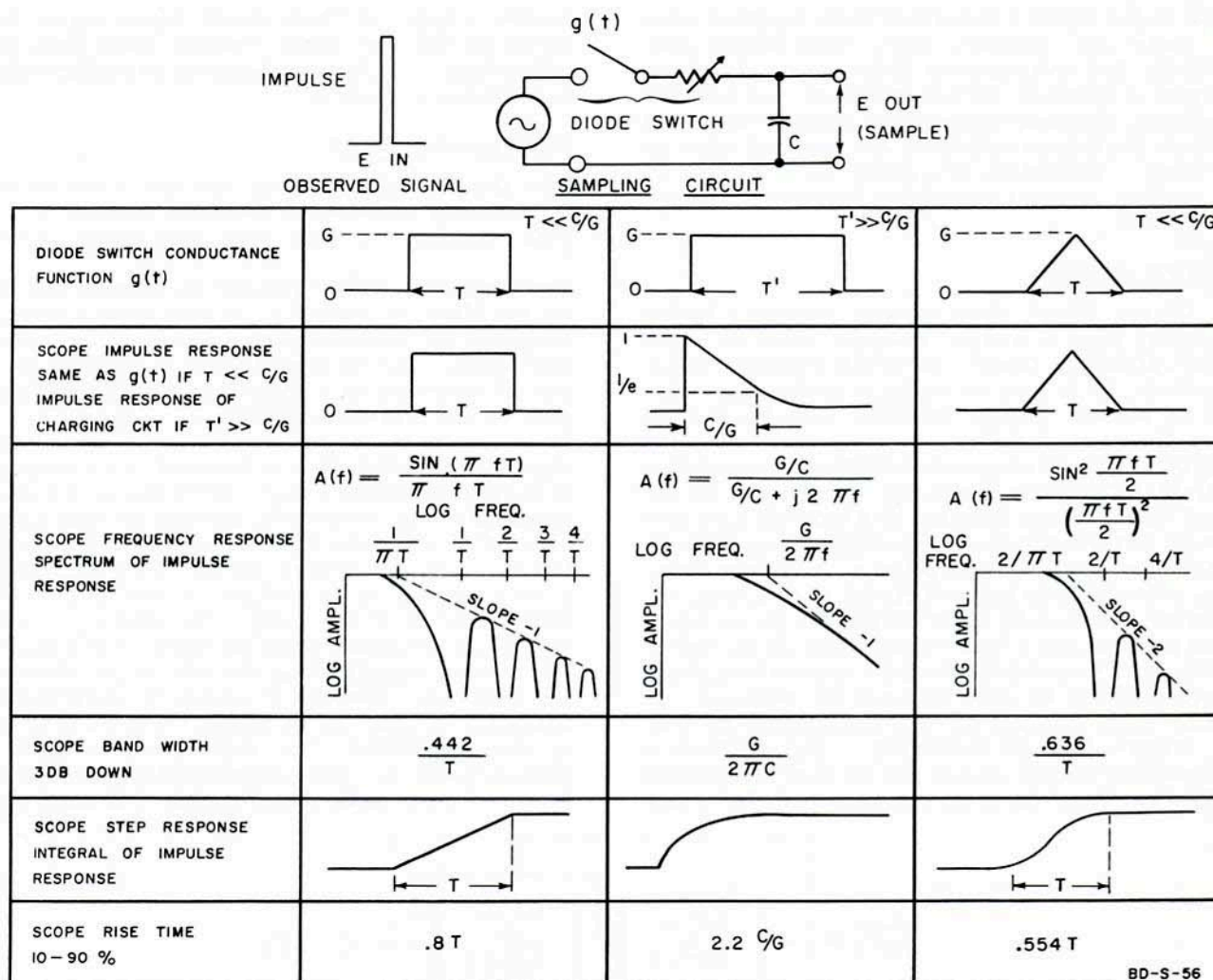
Figure 4. Sampling Oscilloscope Frequency Response
