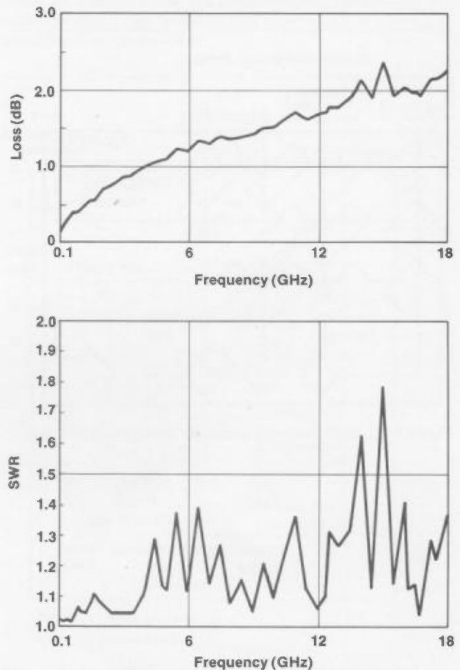
Figure 31. Typical performance of six HP 33311B-C04 4-port switches connected in series.
