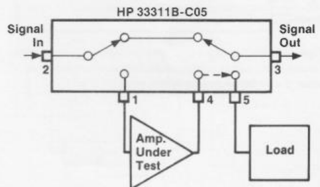
Figure 16. If the device under test is an active component like an amplifier, an external load connected at port 5 provides a load for the amplifier when not inserted in the signal line.
