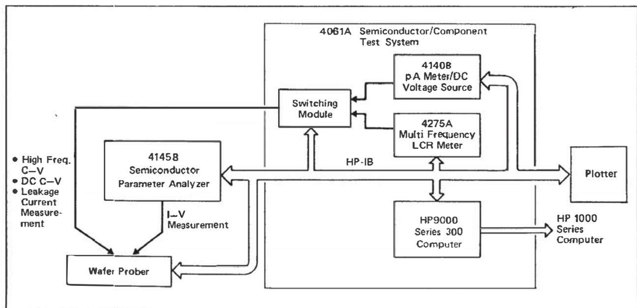
Figure 36. Automatic measurement system for CAD system
