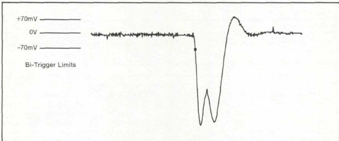
Figure 5. Bi-trigger method used to capture a d\phi/dt pulse from DC-erased media. The dropout width is 256 \mu\text{sec} . Sample rate: 1 \mu\text{sec}/\text{sample} ; bi-trigger limits \pm 70\text{mV} .
