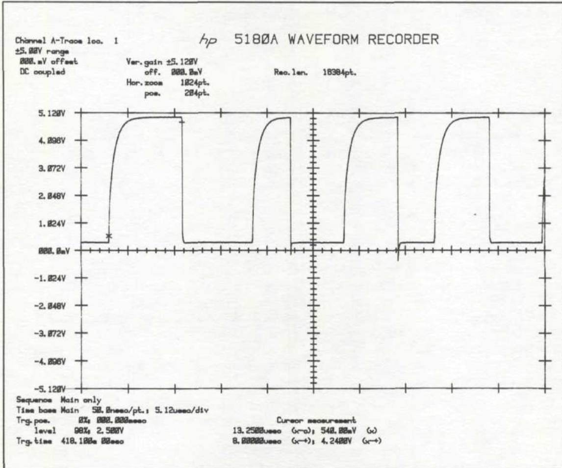
Figure 21. Comparator output waveform for MFM pattern 1011001100110010, having half-pulse widths of 4, 6, and 8 \mu sec.
