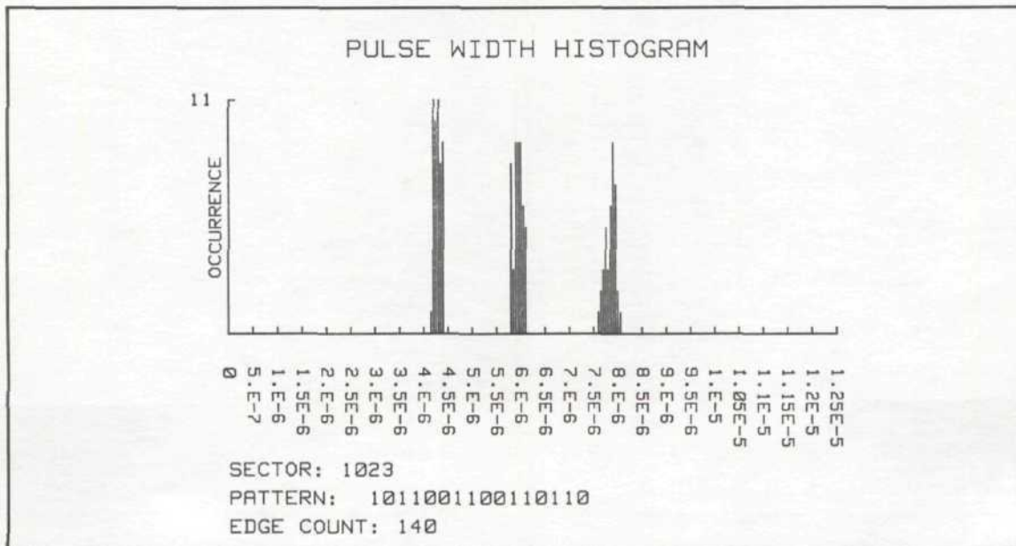
Figure 24. The same MFM pattern used in Figure 23 is written to an inner radius track (sector 1023), producing the pulse width histogram shown. The 8 \mu\text{sec} deviation is wider (450 nsec) than the 8 \mu\text{sec} deviation for an outer radius track (250 nsec, shown in Figure 23).
