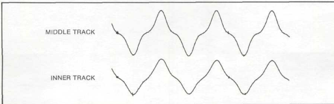
Figure 15. Amplified read pulses from a middle (upper trace) and inner (lower trace) track radius. MFM ... 10101 ... produces the 62.5 KHz signals shown. The two waveshapes are similar, with the inner tracks having wider pulses. Sample period was 50 nsec/sample; record length 1024 points.
