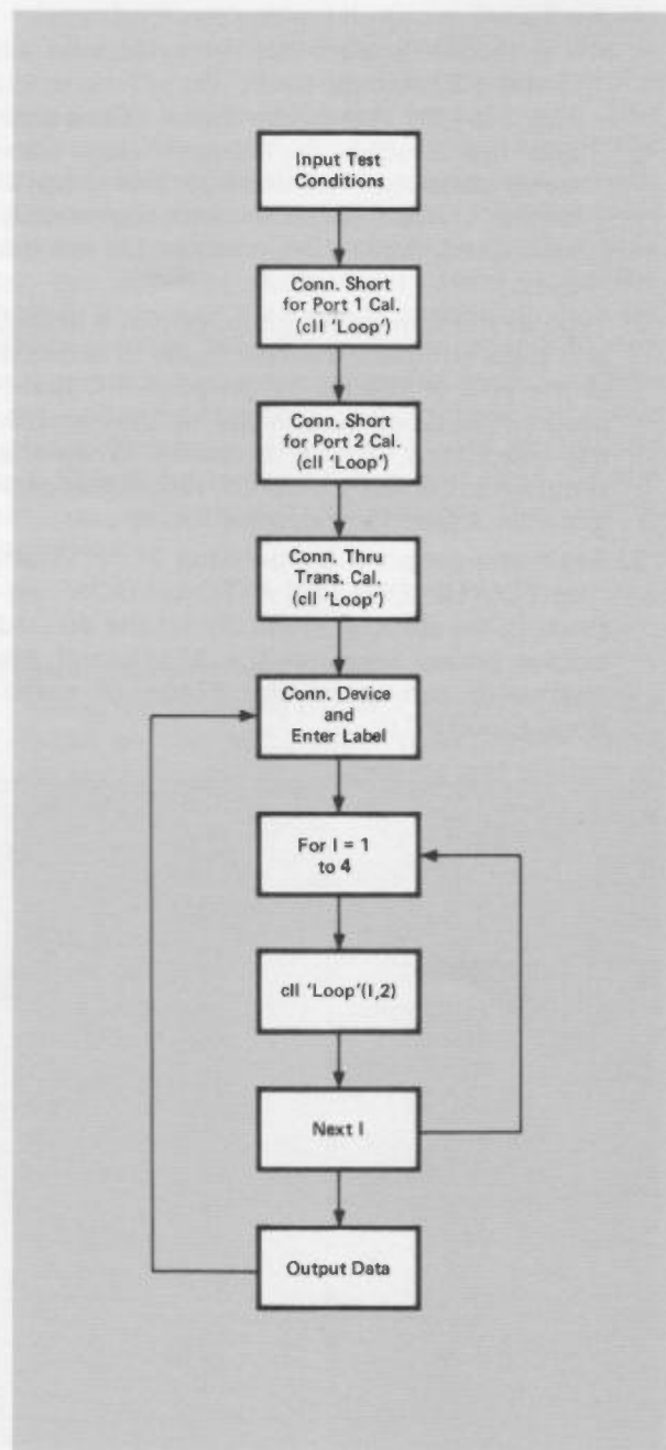
Figure 11. Flowchart of Main Program.
