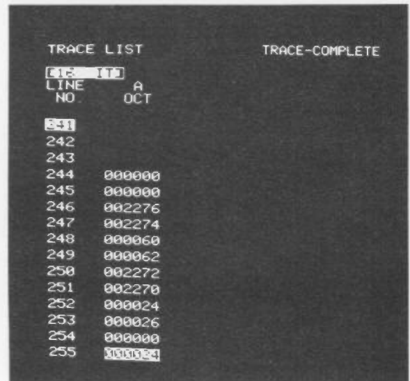
Figure 38. The trace list associated with the timing diagram of figure 37 shows the power fail trap cells on lines 252 and 253.
