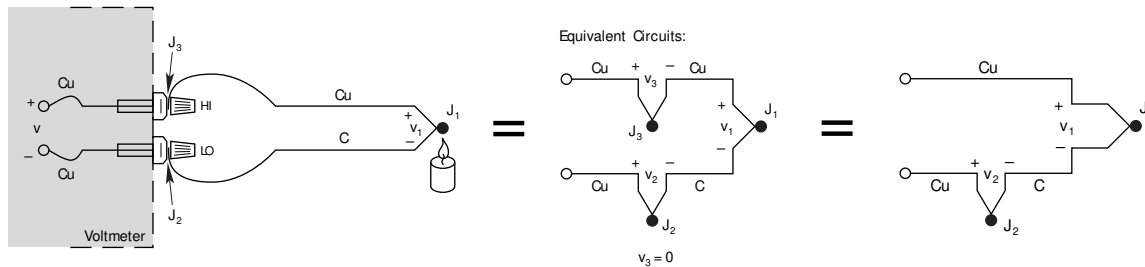
Figure 4 Measuring Junction Voltage with a DVM
