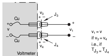
Figure 7 Junction Voltage Cancellation
