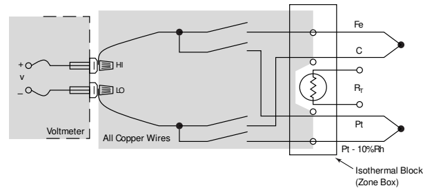
Figure 13 Switching Multiple Thermocouple Types
