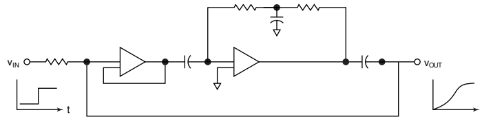
Figure 20 Analog Filter
