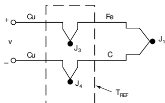
Figure 11 Equivalent Circuit
