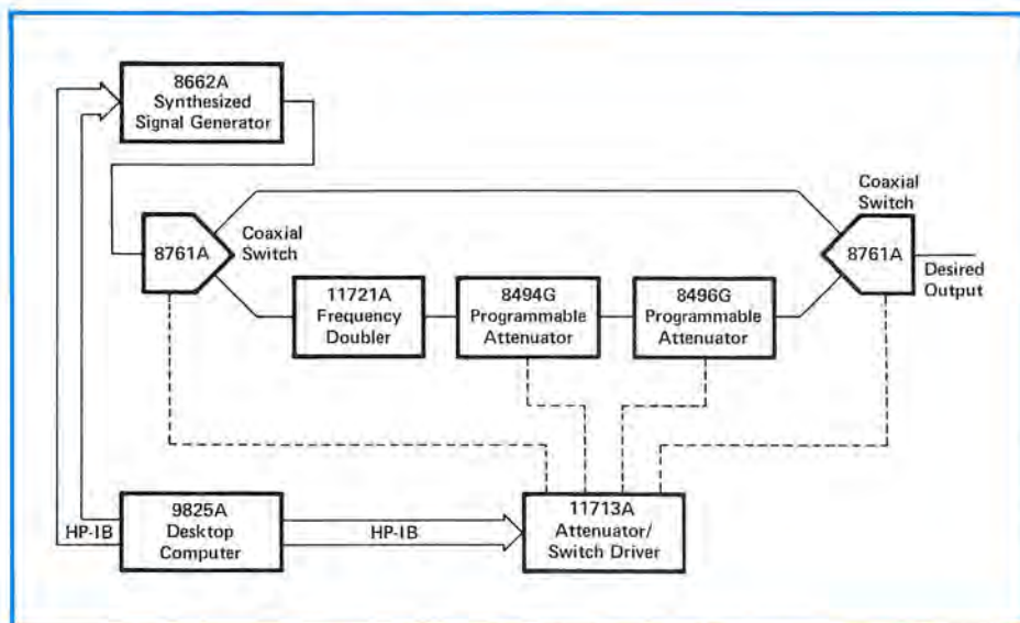
Figure 7. HP-IB System for convenient doubling control.
