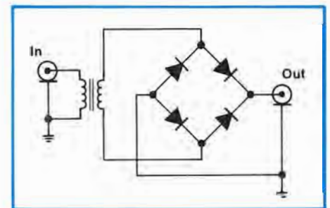
Figure 2. Typical frequency doubler circuit.
