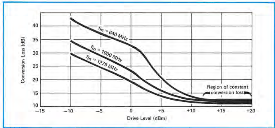
Figure 4. Typical 11721A conversion loss vs. drive level.
