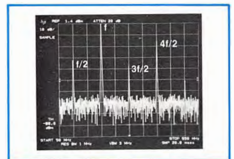
Figure 3. Output spectrum of HP 11721A as seen on HP 8566A Spectrum Analyzer.
