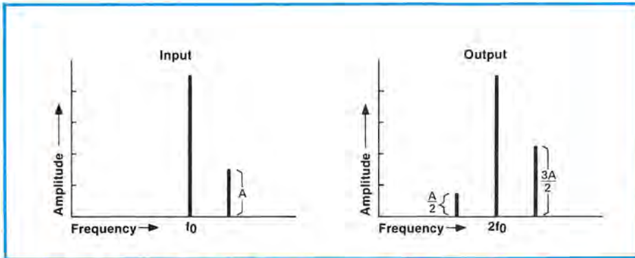
Figure 6. The effect of frequency doubling on spurious signals.
