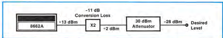
Figure 5. Use of post-doubler attenuation to achieve desired level with full output resolution.
