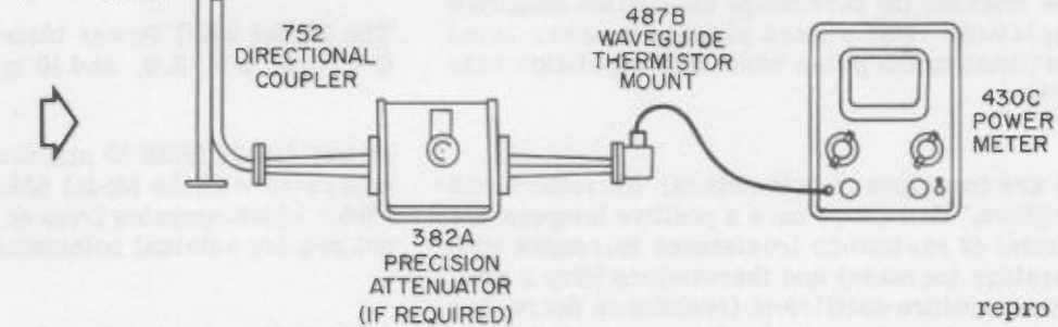
Typical Power Measurement Systems
