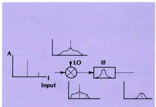
Figure 3. Adjacent Channel Sensitivity
