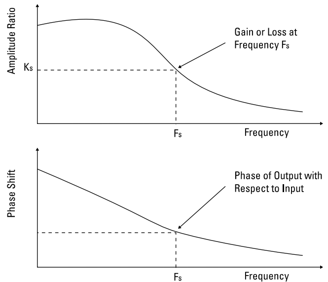
Figure 2.18 The frequency response of a network.
