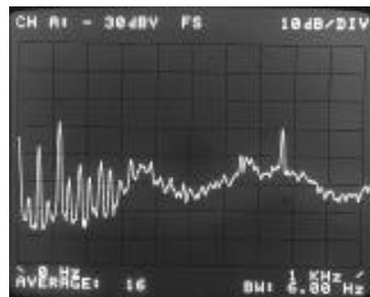
Figure 4.4 Spectrum of electrical motor vibration.
