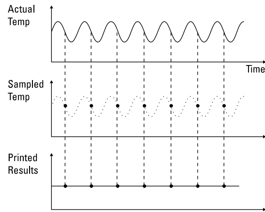
Figure 3.14 Plot of temperature variation of a small part.
