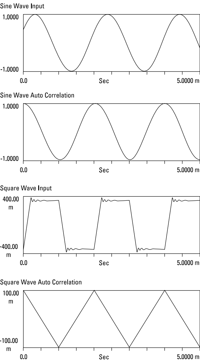
Figure 4.23 Auto correlation of periodic waveforms.
