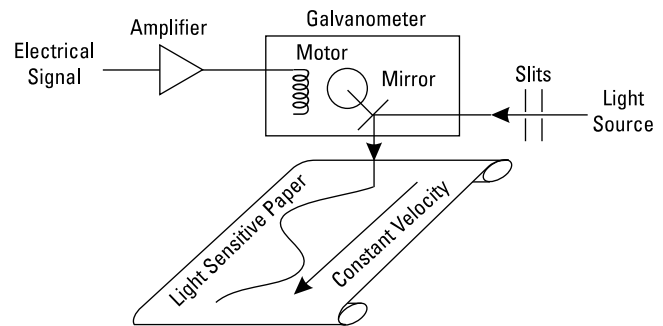
Figure 2.3 Simplified oscilloscope operation.
