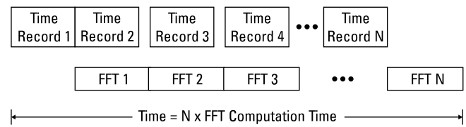
Figure 3.49 RMS averaging time.
