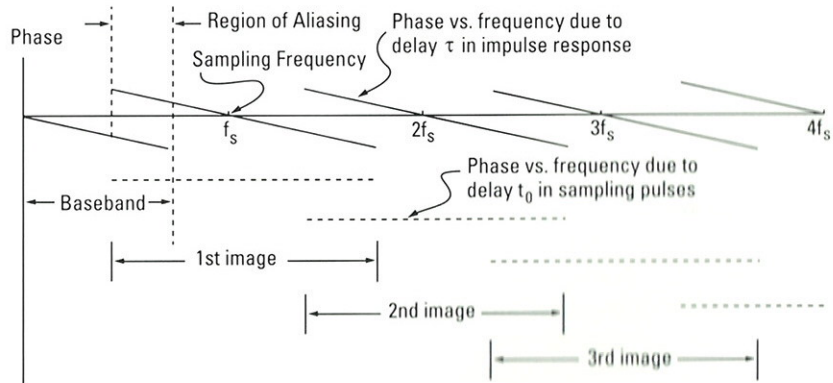
Figure 13: Phase versus frequency due to a time delay in the impulse response, and due to a time delay in the sampling pulses.
