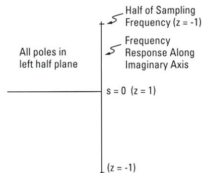
Figure 2: The s -domain, showing the frequency (imaginary) axis.
