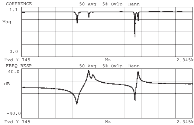
Baseband Measurement
