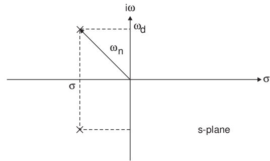
Figure 1.18 S-plane representation
