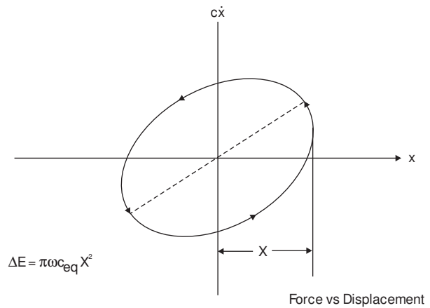
Figure 1.15 Viscous damping energy dissipation
